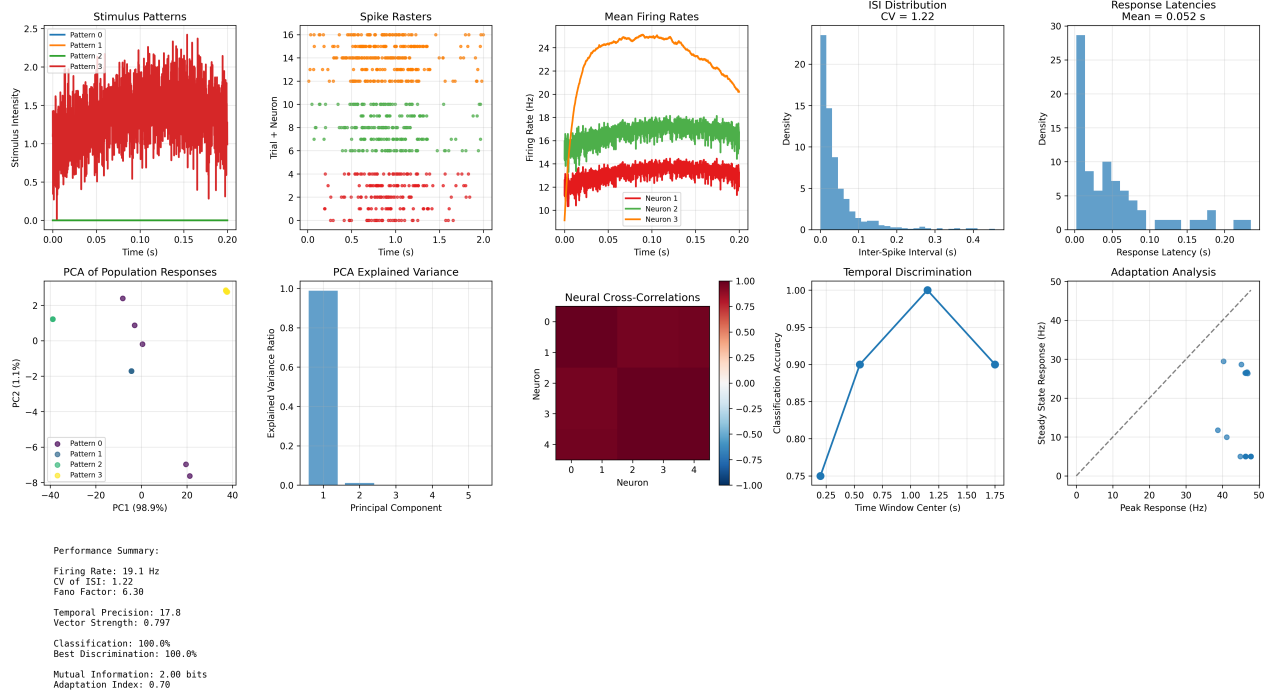
Figure 1: Neural encoding analyses generated deterministically by 'scripts/generate_neural_encoding_analysis.py' using 'src/case_studies/neural_encoding.py'. Panels include spike trains, tempo
