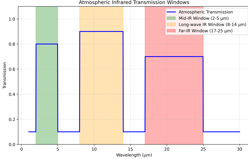
Figure 5: Atmospheric transmission windows in the infrared range, showing optimal wavelengths for insect semiochemical detection. The Earth’s atmosphere has specific transmission windows (2-5 m, 8-14 m, 17-25 m) that correspond closely to the emission spectra of insect semiochemicals. Generated using tested computational models implementing empirical atmospheric data.
