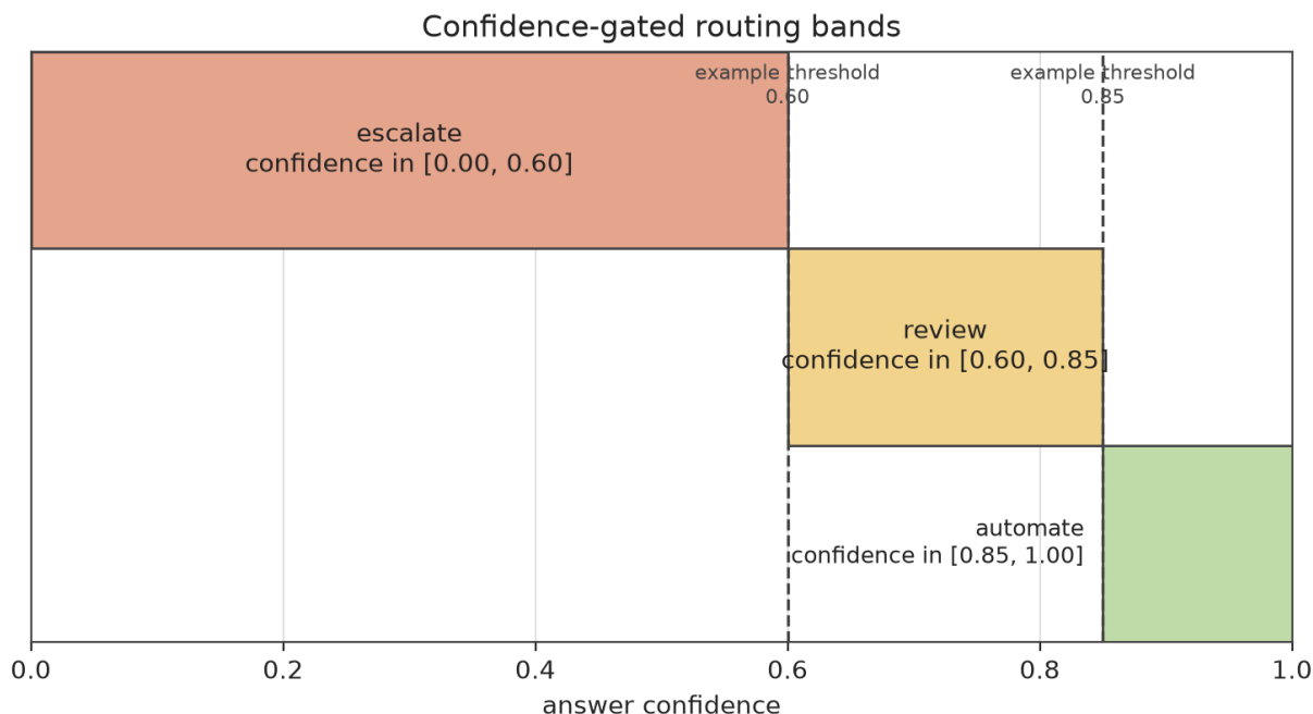
Figure 4: Parametric illustration of confidence-gated routing as implemented by confidence_gate() and route() in src/daf_jeve/compose.py (sec. 4). The horizontal axis is the model-reported confidence on the unit interval; the three horizontal bands assign an action per confidence region — automate above the upper boundary, route to review in the middle band, escalate below the lower boundary. The boundary markers are annotated as example thresholds: the semantics are the bands, not any particular cut points, and the actual thresholds remain policy owned by the caller. This figure is parametric and carries no measured data; sec. 6 measures the latency and calibration properties that make running this policy inline sound.
