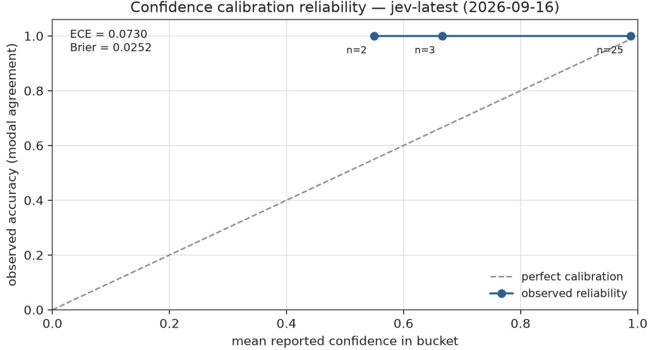
Figure 7: Reliability diagram of choice-answer confidence under the self-consistency proxy, measured by benchmarks/bench_calibration.py over 6 states \times 5 repeats against the jev-latest model on 2026-09-16. Each point is a confidence bucket plotting mean reported confidence against proxy accuracy, where proxy accuracy is agreement with the modal choice across repeats of the same state; the dashed diagonal marks perfect agreement between stated confidence and observed proxy accuracy. Because the proxy scores self-agreement rather than verified correctness, proximity to the diagonal indicates consistency between stated confidence and repeat-stable behaviour — not truthfulness about the world. Aggregate scores are tabulated in tbl. 3 .
