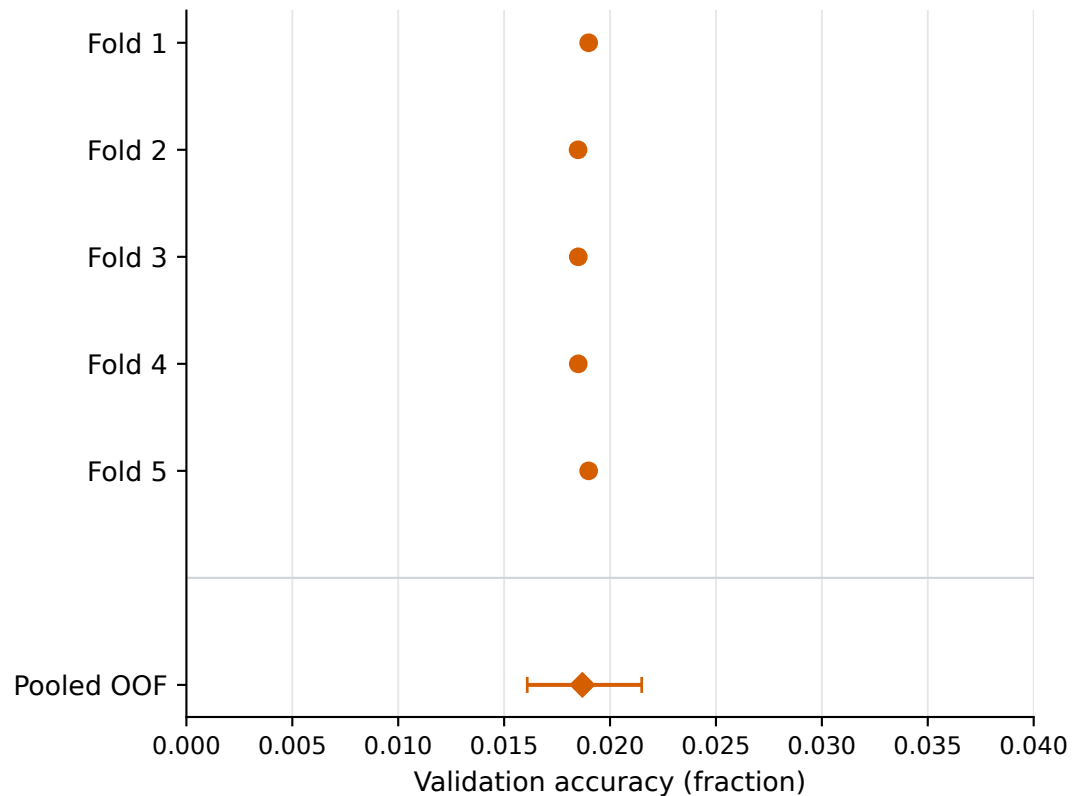
Training prior
