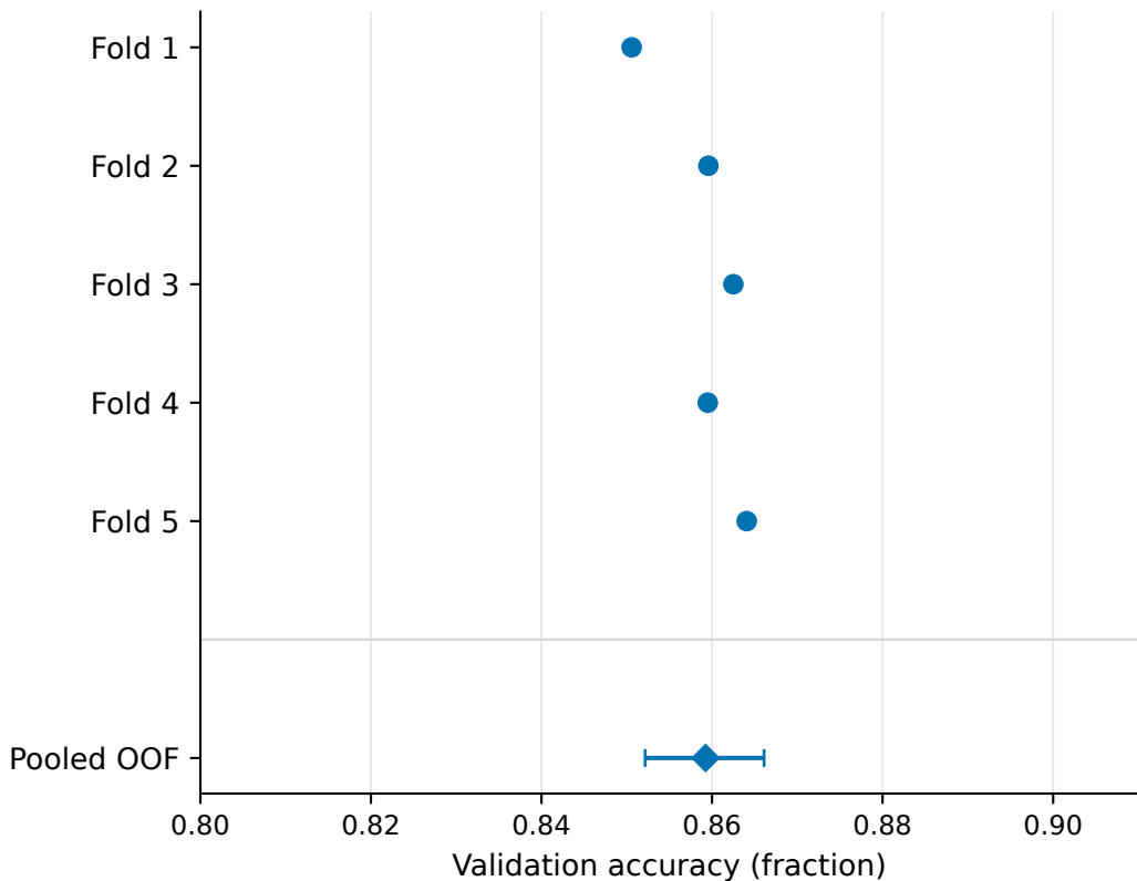
TF-IDF + logistic (C=1)
