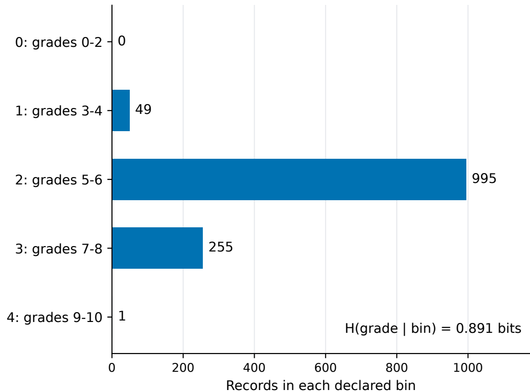
b Canonical test support
