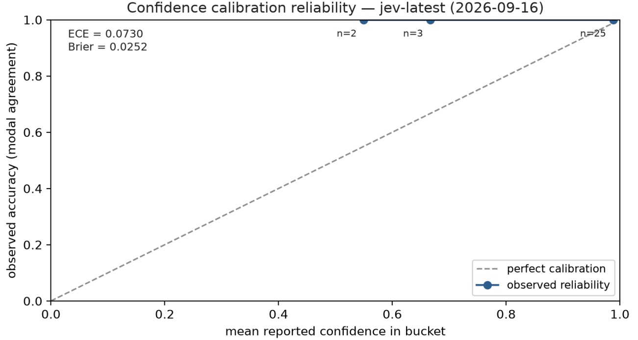
Figure 6: Reliability diagram of choice-answer confidence under the self-consistency proxy, measured by benchmarks/bench_calibration.py over 6 states \times 5 repeats against the jev-latest model on 2026-09-16. Each point is a confidence bucket plotting mean reported confidence against proxy accuracy, where proxy accuracy is agreement with the modal choice across repeats. Because the proxy scores self-agreement rather than verified correctness, the diagonal indicates consistency between stated confidence and repeat-stable behaviour — not truthfulness.
