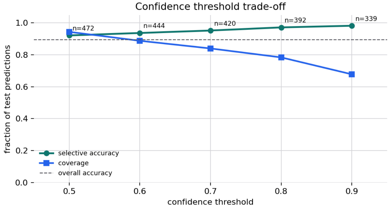
Figure 21: Confidence-threshold trade-off for exp-mlp-tanh-64 from output/data/ml_statistical_summary.json; the plot compares retained coverage, selective accuracy, and the unthresholded accepted-candidate accuracy on the fixed local split. Generation method: Confidence-threshold coverage and selective-accuracy line chart. Registry metadata records the generation method, source artifact, and claim boundary for validation.
