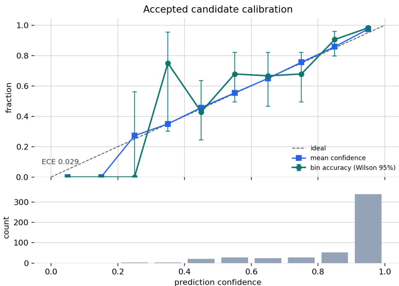
Figure 13: Reliability curve for exp-mlp-tanh-64 from output/data/ml_calibration_report.json; expected calibration error and bin counts summarize the accepted candidate on the fixed local test split. Generation method: Reliability curve with confidence-bin support histogram. Registry metadata records the generation method, source artifact, and claim boundary for validation.
