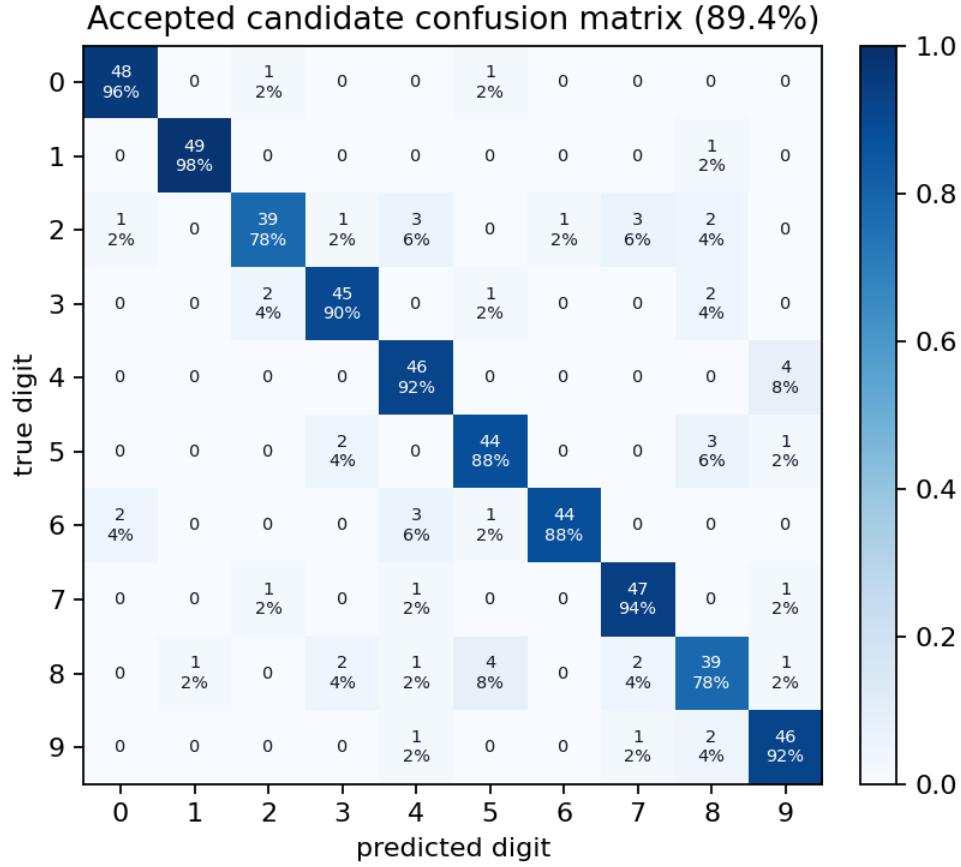
Figure 6: Accepted-candidate confusion matrix for exp-mlp-tanh-64 on the fixed MNIST handwritten digit database test split, sourced from output/data/ml_confusion_matrix.csv; it diagnoses the selected run, not general full-dataset performance. Generation method: Row-normalized heatmap with cell counts and row percentages. Registry meta-data records the generation method, source artifact, and claim boundary for validation.
