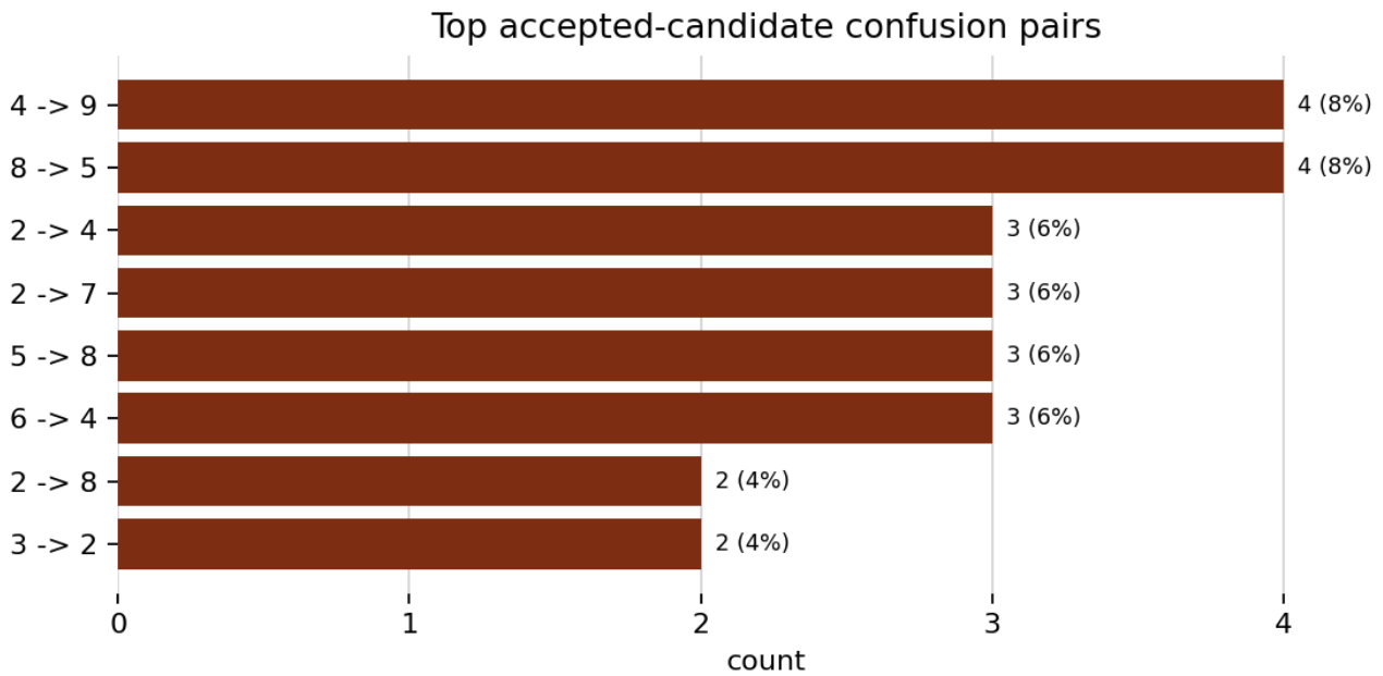
Figure 15: Top non-diagonal confusion pairs for exp-mlp-tanh-64, sourced from output/data/ml_classification_diagnostics.json; the bars highlight which local digit pairs account for accepted-candidate errors. Generation method: Ranked off-diagonal confusion-pair bars with true-class error rates. Registry metadata records the generation method, source artifact, and claim boundary for validation.
