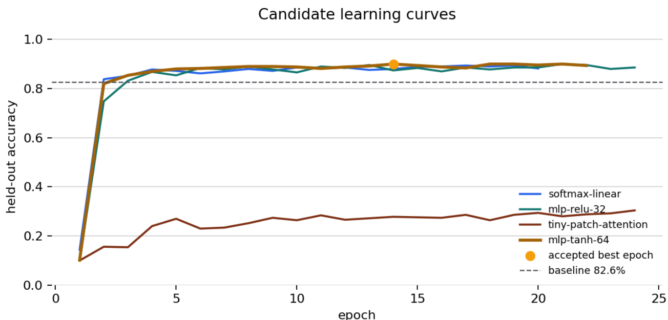
Figure 8: Epoch-level held-out accuracy curves for evaluated candidates from output/data/ml_training_history.csv; the accepted curve is visually emphasized for exp-mlp-tanh-64. Generation method: Epoch-level held-out accuracy lines with accepted best-epoch marker. Registry metadata records the generation method, source artifact, and claim boundary for validation.
