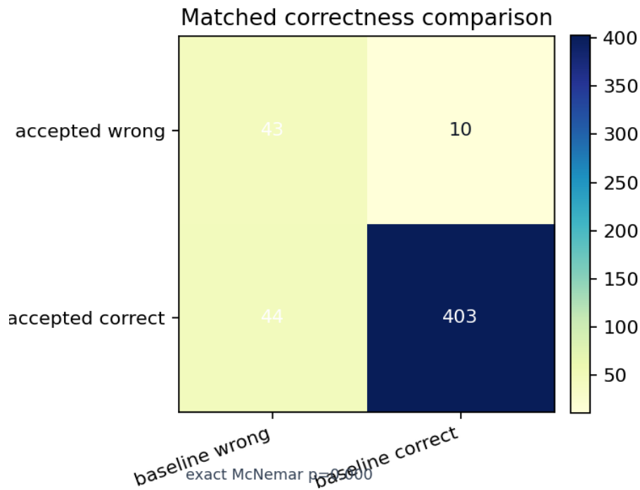
Figure 20: Matched correctness comparison between exp-mlp-tanh-64 and the nearest_centroid_baseline baseline from output/data/ml_paired_comparison.json; discordant cells support the paired test summary. Generation method: Matched accepted-versus-baseline correctness heatmap. Registry metadata records the generation method, source artifact, and claim boundary for validation.
