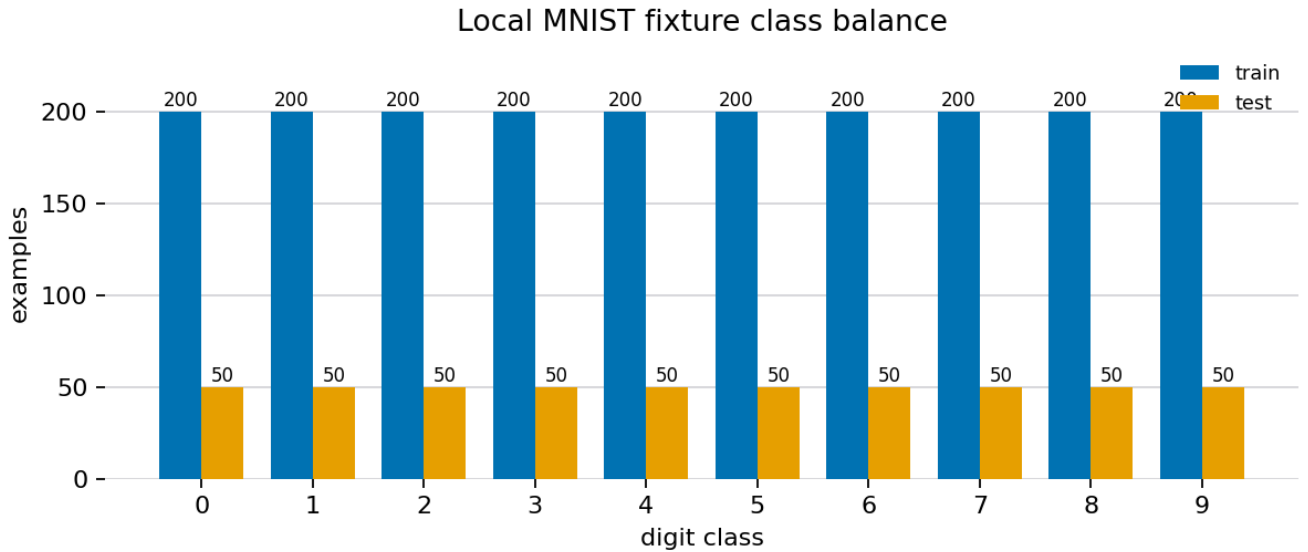
Figure 1: Train and test class counts from output/data/ml_class_balance.json ; the local fixture contains 2000 train and 500 test examples across 10 classes. Generation method: Grouped train/test class-count bars from the local MNIST fixture. Registry metadata records the generation method, source artifact, and claim boundary for validation.
