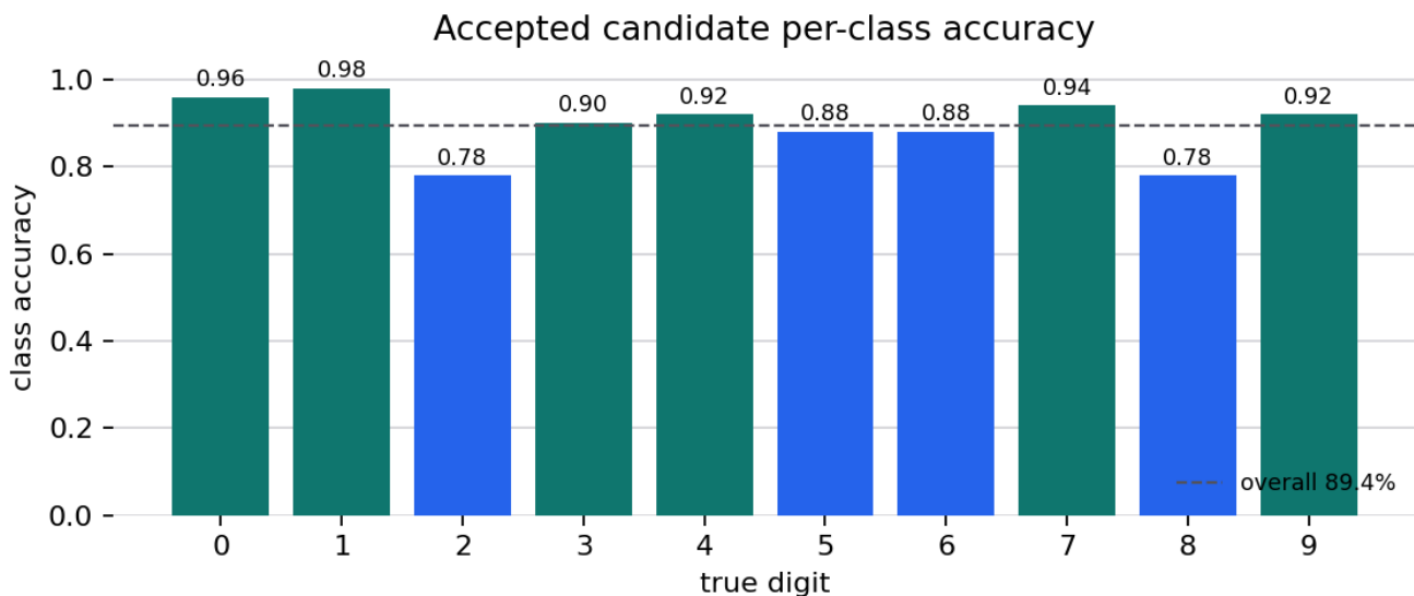
Figure 7: Per-class accuracy for exp-mlp-tanh-64, computed from output/data/ml_confusion_matrix.csv; variation across digits is a run diagnostic for the fixed local test split. Generation method: Per-class accuracy bars computed from the confusion matrix diagonal. Registry metadata records the generation method, source artifact, and claim boundary for validation.
