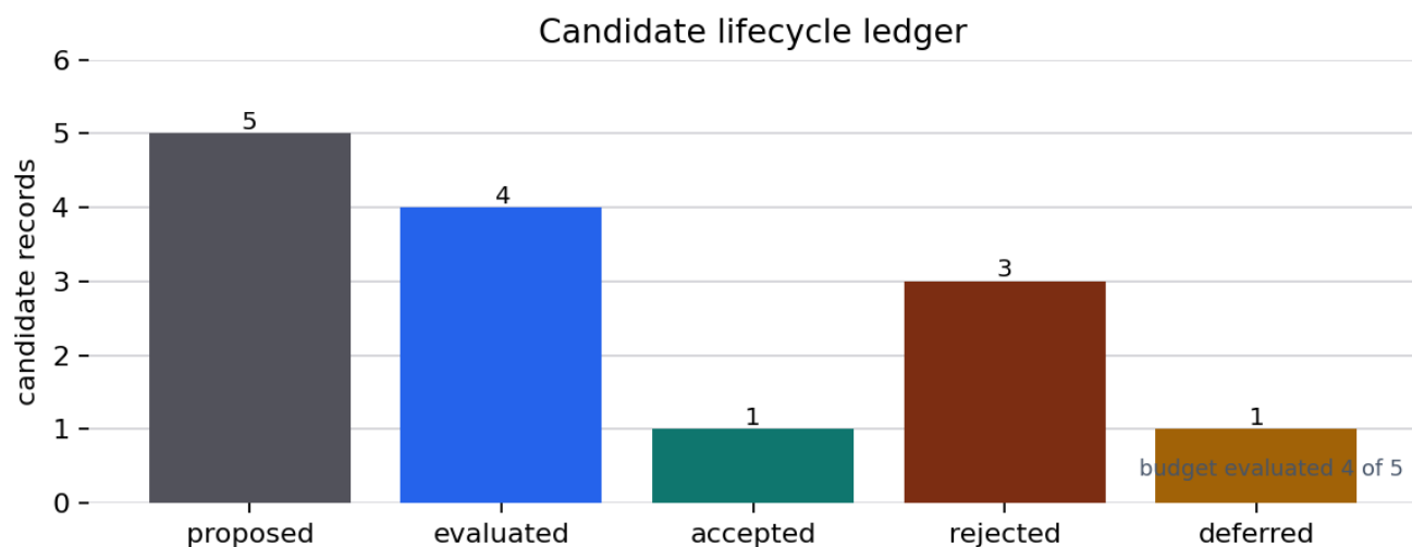
Figure 12: Candidate lifecycle ledger from output/data/ml_candidate_ledger.json: 4 evaluated out of 5 proposed candidates, with deferred proposals kept visible instead of executed automatically. Generation method: Candidate lifecycle status-count bar chart. Registry metadata records the generation method, source artifact, and claim boundary for validation.
