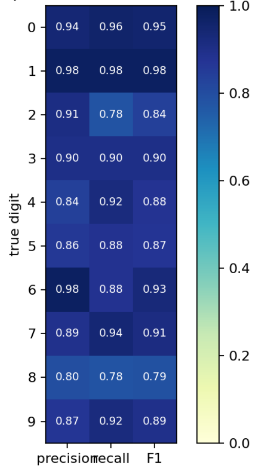
Accepted candidate class metrics
