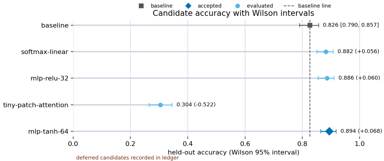
Figure 4: Held-out accuracy with Wilson intervals for the baseline and evaluated candidates from output/data/ml_candidate_intervals.json; accepted candidate exp-mlp-tanh-64 improves accuracy from 82.6% to 89.4% on the fixed subset, with deferred proposals kept in the candidate ledger. Generation method: Lollipop accuracy comparison with Wilson interval error bars and direct labels. Registry metadata records the generation method, source artifact, and claim boundary for validation.
