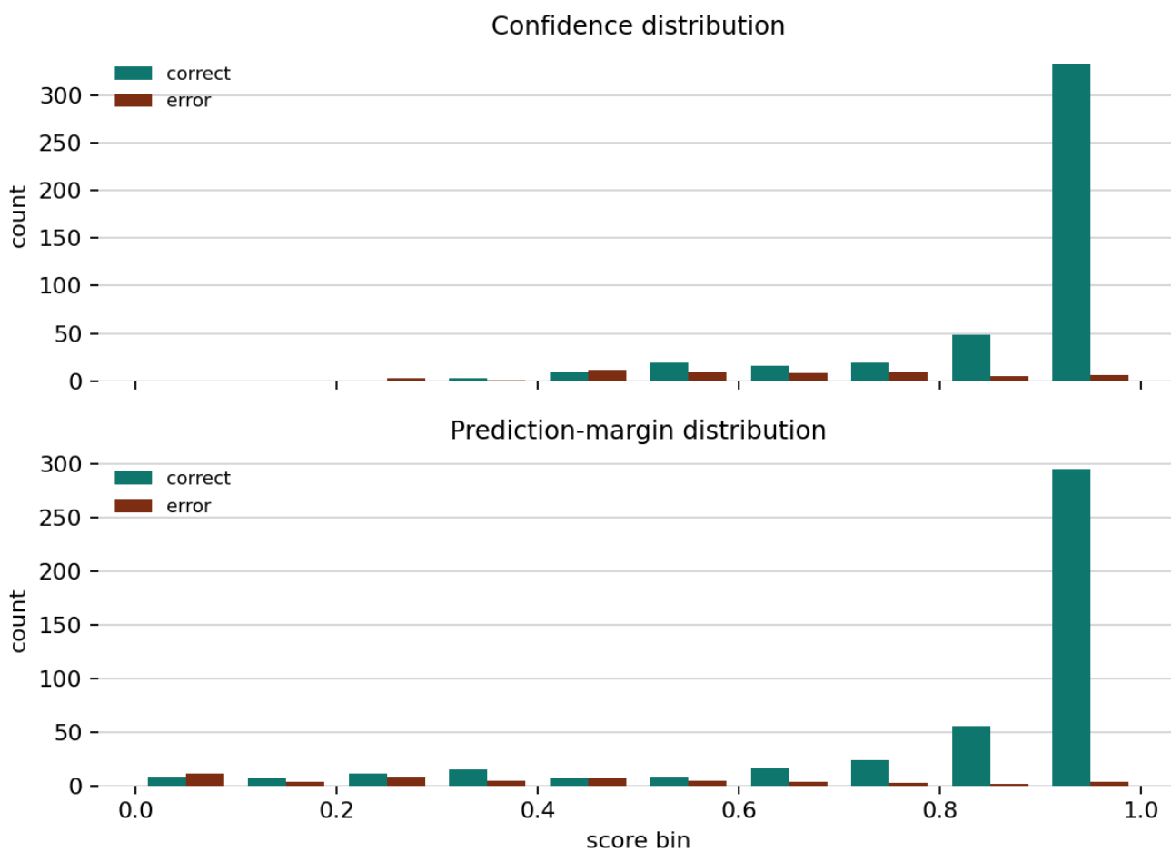
Figure 18: Confidence and prediction-margin histograms for exp-mlp-tanh-64 from output/data/ml_probability_diagnostics.json; the figure separates correct and incorrect local test predictions. Generation method: Confidence and margin histograms split by correctness. Registry metadata records the generation method, source artifact, and claim boundary for validation.
