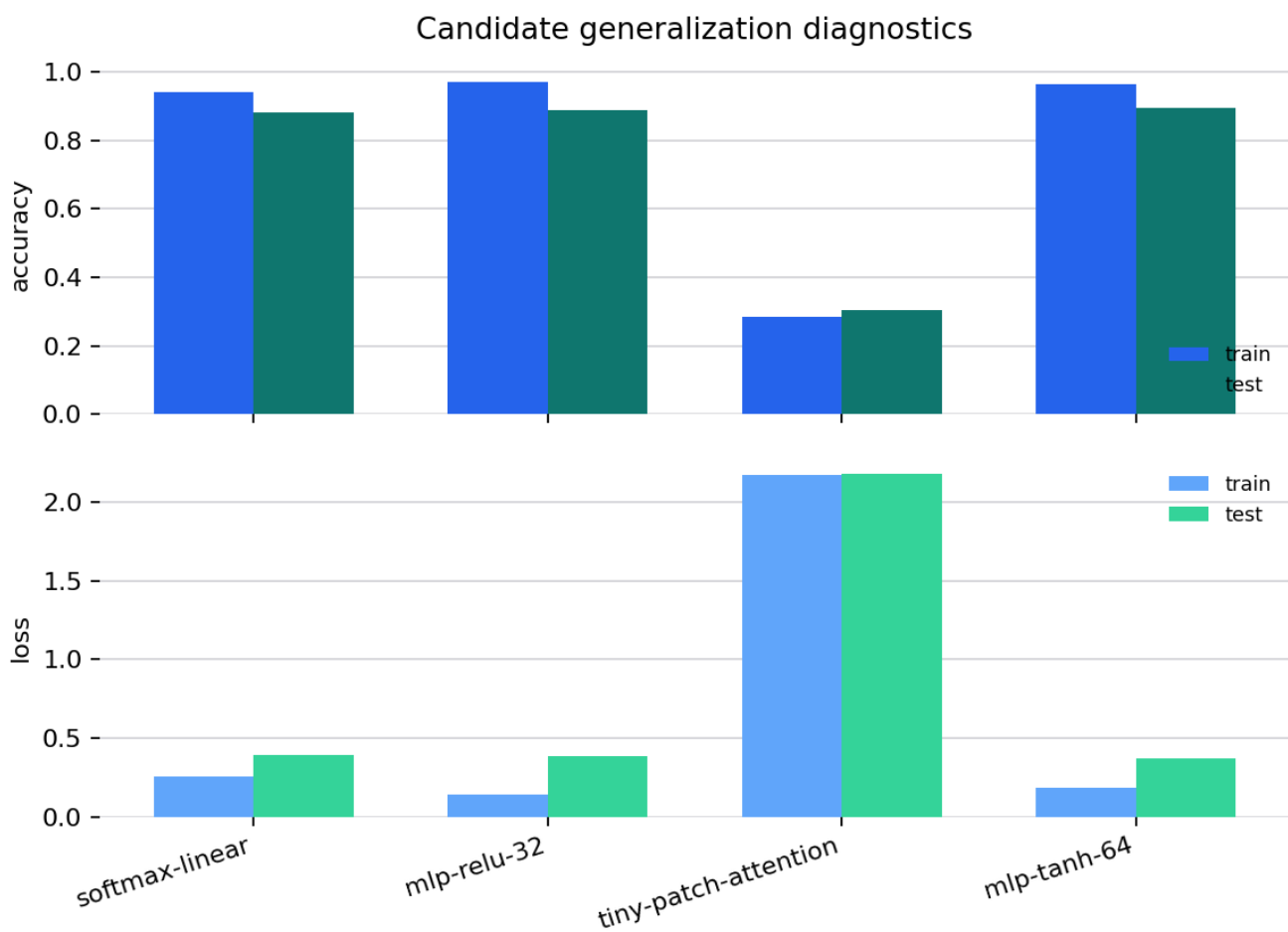
Figure 16: Train/test accuracy and loss for evaluated candidates from output/data/ml_classification_diagnostics.json; the plot exposes local generalization gaps without claiming full-dataset behavior. Generation method: Grouped train/test accuracy and loss bars by evaluated candidate. Registry metadata records the generation method, source artifact, and claim boundary for validation.
