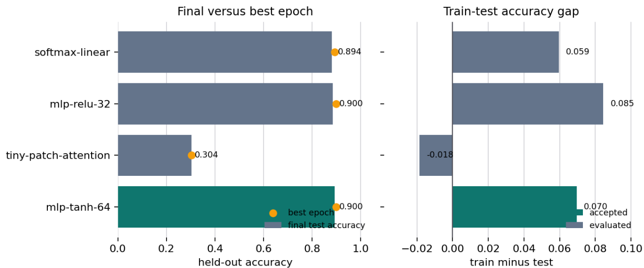
Figure 9: Configured-training dynamics for evaluated candidates from output/data/ml_training_diagnostics.json; exp-mlp-tanh-64 is highlighted while best-epoch markers and train-test gaps remain bounded to the local run. Generation method: Final and best-epoch accuracy bars plus train-test gap bars. Registry metadata records the generation method, source artifact, and claim boundary for validation.
