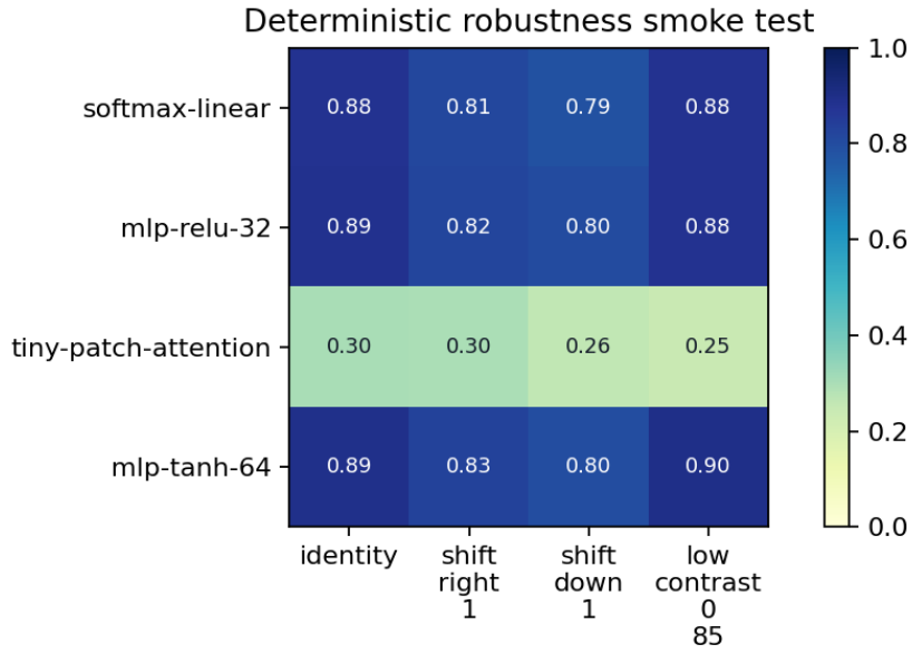
Figure 17: Accuracy for evaluated candidates under identity, one-pixel shifts, and low contrast from output/data/ml_robustness_report.json ; the deterministic transforms provide a bounded smoke test only. Generation method: Candidate-by-transform accuracy heatmap for deterministic perturbations. Registry metadata records the generation method, source artifact, and claim boundary for validation.
