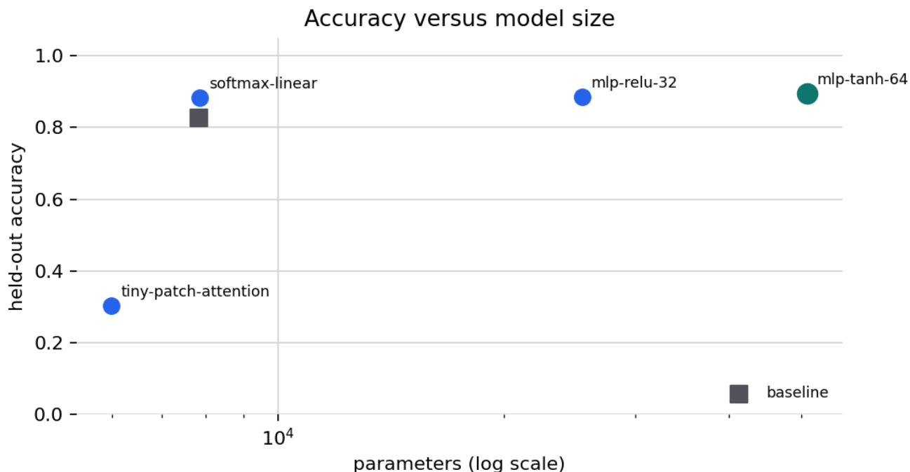
Figure 10: Parameter-count versus held-out accuracy for the baseline and evaluated candidates from output/data/ml_task_results.json; the accepted candidate is highlighted without claiming a general scaling law. Generation method: Log-parameter scatter plot against held-out accuracy. Registry metadata records the generation method, source artifact, and claim boundary for validation.
