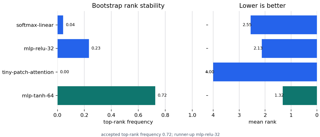
Figure 5: Rank-stability summary for exp-mlp-tanh-64 from output/data/ml_candidate_rank_stability.json; deterministic local bootstrap resampling shows how often each evaluated candidate ranks first under the fixed test split. Generation method: Bootstrap top-rank frequency and mean-rank comparison. Registry metadata records the generation method, source artifact, and claim boundary for validation.
