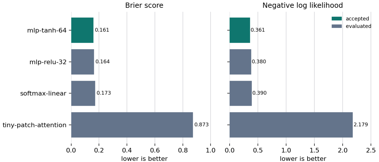
Figure 22: Brier score and negative log likelihood for evaluated candidates from output/data/ml_statistical_summary.json; lower values indicate better probability quality within the configured local run, and the accepted candidate is highlighted. Generation method: Brier score and negative-log-likelihood bar comparison. Registry metadata records the generation method, source artifact, and claim boundary for validation.
