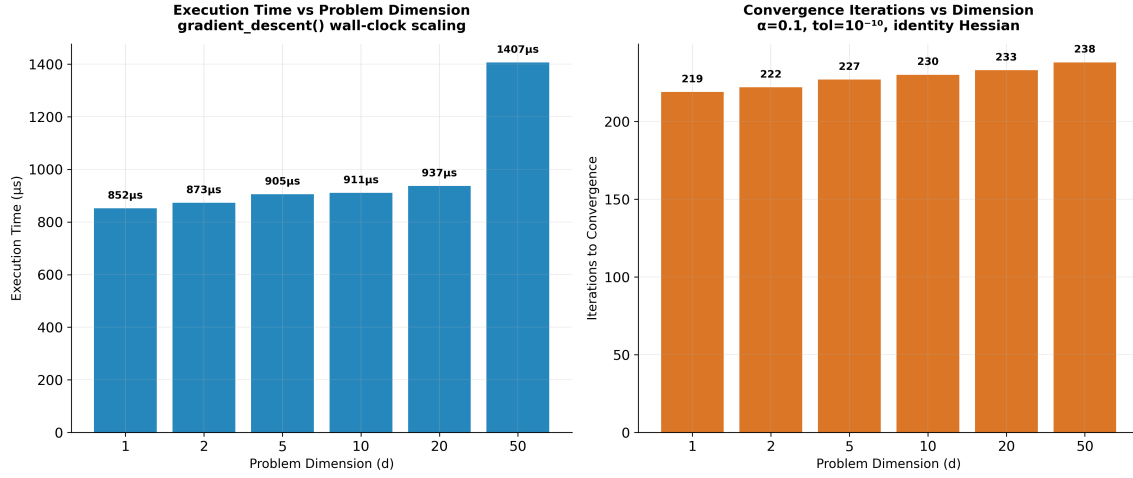
Figure 6: Dimensional scaling from generate_benchmark_visualization() . Dimensions d \in \{1, 2, 5, 10, 20, 50\} run on identity-Hessian quadratics with \alpha = 0.1 and gradient tolerance 10^{-10} (both hardcoded in the script for benchmark stability). Left: mean wall-clock time per gradient_descent() call ( \mu s ). The flat regime at d \leq 20 reflects per-iteration overhead (Python dispatch, NumPy bookkeeping); the upturn at d = 50 shows the O(d) matrix-vector cost beginning to dominate. Right: iterations-to-convergence rises only modestly across two decades of d ( 219 \rightarrow 238 ). This near-invariance is expected: \kappa(I_d) = 1 regardless of dimension, so the contraction factor \rho = |1 - \alpha| = 0.9 is identical for every d , and only the per-coordinate residual norm grows mildly.
