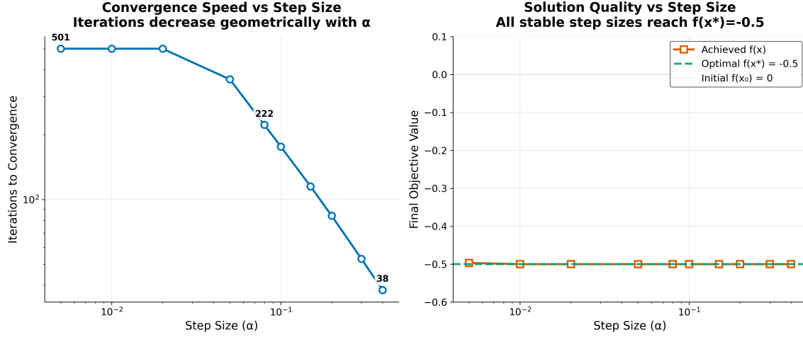
Figure 3: Sensitivity sweep produced by generate_step_size_sensitivity_plot() over an independent dense grid \alpha \in [0.005, 0.4] (15 points), distinct from the discrete experiment.step_sizes used elsewhere in this section. Left: iterations to convergence on log-log axes — the curve drops sharply from 501 iterations at the smallest \alpha (the max_iterations cap in this sub-experiment) to 38 iterations at \alpha = 0.4 , illustrating the geometric speedup as \rho(\alpha) = |1 - \alpha| shrinks. Right: final f(x) versus \alpha with horizontal reference lines at f(x_0) = 0 (initial) and f(x^*) = -0.5 (analytic optimum); every \alpha in this stable window lands on the optimum.
