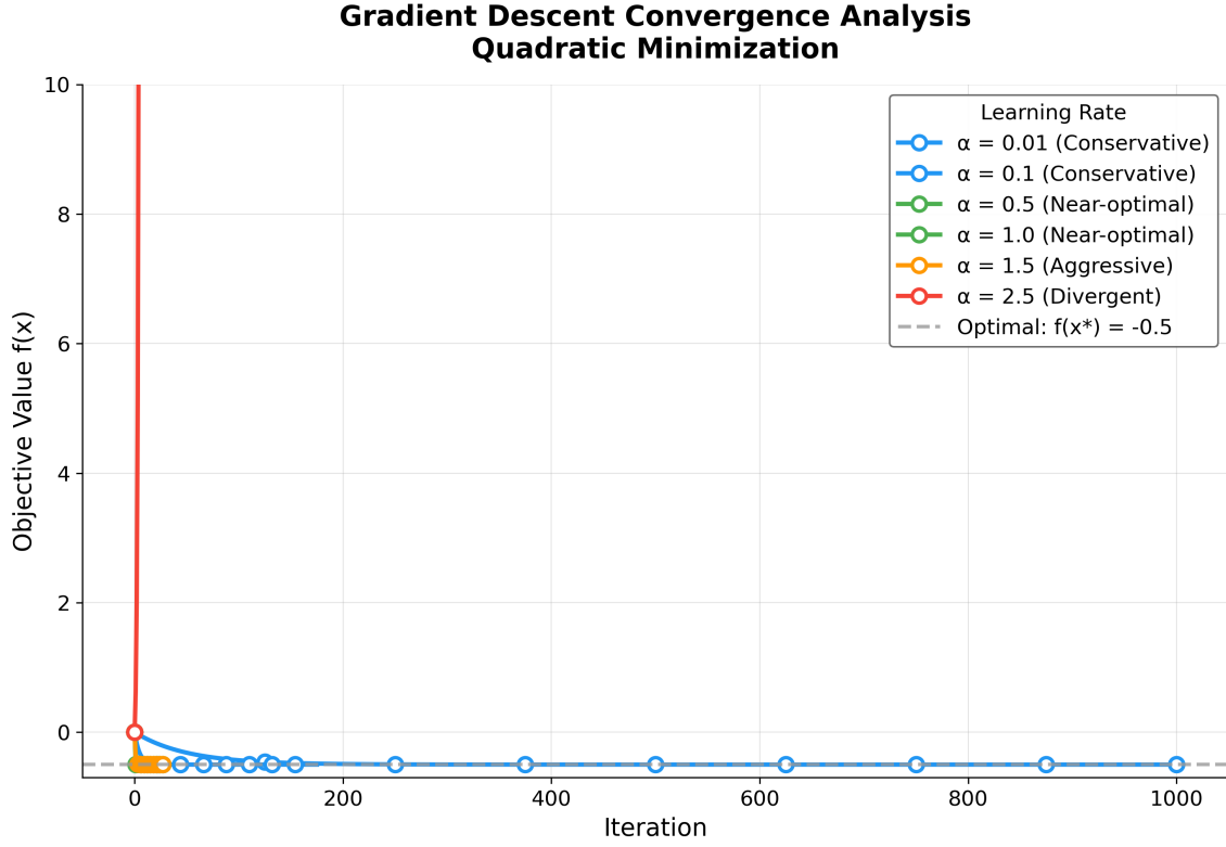
Figure 2: Objective value f(x_k) = \frac{1}{2}x_k^2 - x_k versus iteration k for gradient descent at six step sizes (legend colours follow the agency taxonomy in sec. 4: blue = conservative, green = near-optimal, orange = aggressive, red = divergent). Trajectories are produced by simulate_trajectory() in src/optimizer.py , which calls the same gradient_descent() used in tbl. 1; the upper bound on the y-axis clips the divergent \alpha = 2.5 curve so that stable trajectories remain visible. Dashed grey reference line marks the analytic optimum f(x^*) = -0.5 . Fastest configuration in this experiment: \alpha = 1.0 converges in 1 iteration(s).
