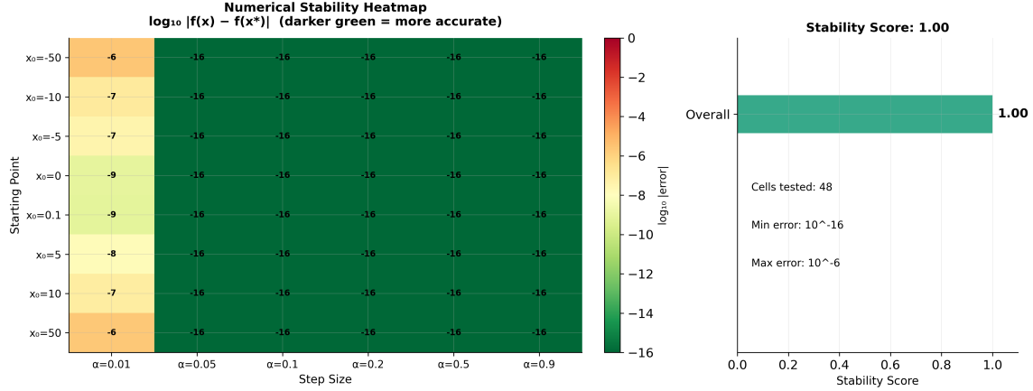
Figure 7: Numerical stability heatmap from generate_stability_visualization() . Each cell shows \log_{10} |f(x) - f(x^*)| at termination for one (starting point x_0 , step size \alpha ) combination, evaluated by gradient_descent() over the 8-by-6 grid (48 cells). The leftmost column ( \alpha = 0.01 , conservative) reaches only 10^{-6} to 10^{-9} within the iteration cap, while every other column saturates at machine precision ( 10^{-16} ) regardless of how far x_0 starts from the optimum (range [-50, 50] ). The right panel summarises this uniformity as the aggregate stability score of 1.00/1.00 returned by infrastructure.scientific.stability.check_numerical_stability() , which exercises the same objective with extreme inputs ( \text{NaN} , \pm\infty , \pm 10^{10} ).
