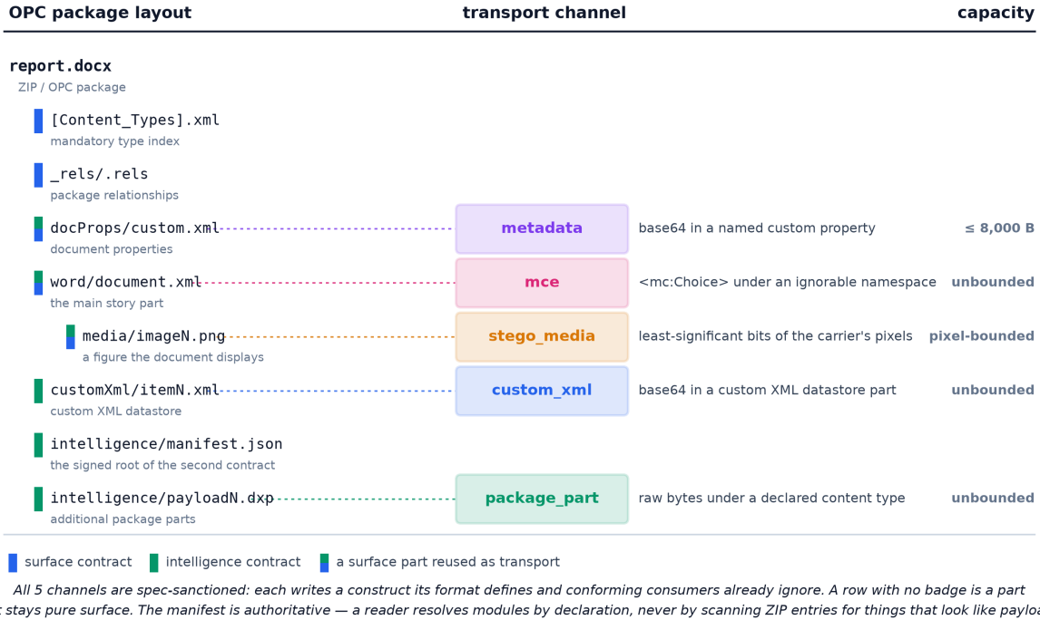
Figure 1. The package tree with every transport channel drawn on the row of the part it writes into. A blue marker is a part the surface contract requires, a green one a part only docxplus reads, and a split marker a required part reused as transport — which is how three of the 5 channels carry a payload without adding any part a conforming reader would find surprising. Rows with no badge carry nothing. Capacities are read from the live code constants.
