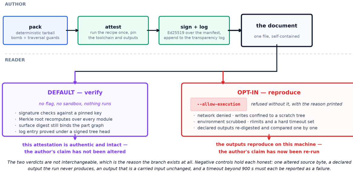
Figure 3. Authoring runs left to right and ends at one self-contained file; what a reader does with that file forks. The default branch is entirely cryptographic and executes nothing. The other requires an explicit flag and re-runs the attested command under confinement. The fork exists because the two verdicts are not interchangeable: one says the author's claim has not been altered, the other says it reproduces on this machine, and neither substitutes for the other.
