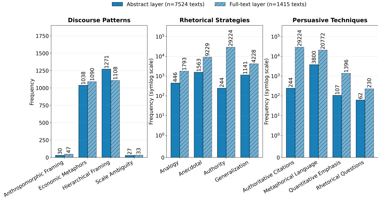
Figure 16. Lexical discourse, rhetorical and persuasive-pattern counts, with analyzed-text counts shown in the legend. PMC uses an explicitly bounded text sample. Raw frequencies depend on sample size and text length and must not be read as normalized prevalence or human-validated author intent.
