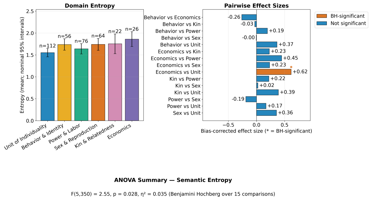
Figure 13. Headline valid-entropy descriptives with nominal intervals, bias-corrected standardized differences, and exploratory ANOVA. Bar annotations report valid term counts; overlapping domain memberships and shared document contexts limit population inference.
