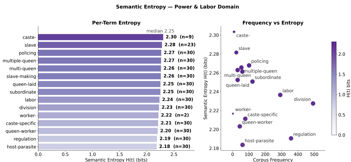
Figure 12. Power and Labor terms ranked by attached context-cluster entropy, with corpus frequency and short extraction-context counts. Sentence-context entropy and the plotted extraction-window counts use different context definitions. Cluster entropy is not an independently validated ambiguity measure.
