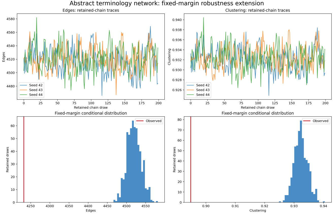
Figure 2. Fixed-margin comparison for the abstract terminology network. Top: retained-chain traces of projected edge count and mean local clustering for 3 seeds. Bottom: distributions of the 600 retained draws, with the observed value marked. Every draw preserves each abstract’s selected-term count and each term’s document frequency. The reference is conditional on the frequency-ranked vocabulary and the convenience corpus.
