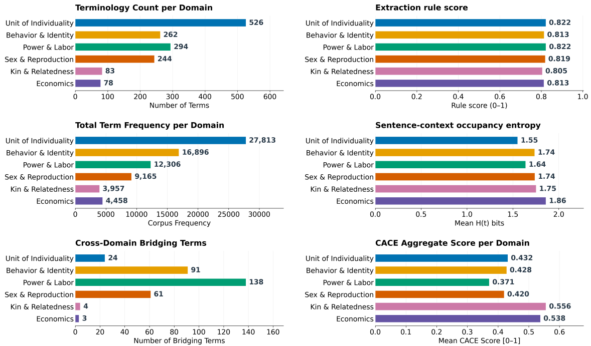
Figure 4. Six descriptive panels show distinct term counts, mean extraction confidence, total frequency, mean successfully computed sentence-context entropy, bridging counts, and heuristic CACE means over up to fifty selected terms per domain. Extraction confidence is a configured score rather than calibrated classification accuracy. Entropy and CACE sample definitions are specified in Methods; missing entropy does not establish zero ambiguity.
