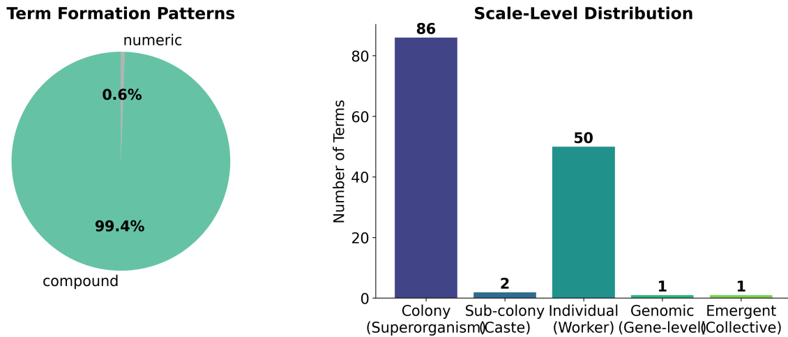
Figure 8. Terminology patterns in the Unit of Individuality domain, computed at build time from the domain’s terms in the headline abstract layer (1907 open-access PubMed abstracts; output/data/domain_statistics.json ). Left: term-formation patterns (the part-of-speech structure of the domain’s terms) as a pie chart, with slice angles proportional to pattern counts and percentages annotated. Right: number of domain terms whose names match keyword groups for five biological scales—Colony (Superorganism), Sub-colony (Caste), Individual (Worker), Genomic (Gene-level), and Emergent (Collective)—as a bar chart with counts annotated; counts are floored at one for display, so a near-zero scale is indistinguishable from a single match. Colony-level terms such as “colony” and “superorganism” populate the colony-scale group; the distribution across scales grounds the scale ambiguities discussed in the text.
