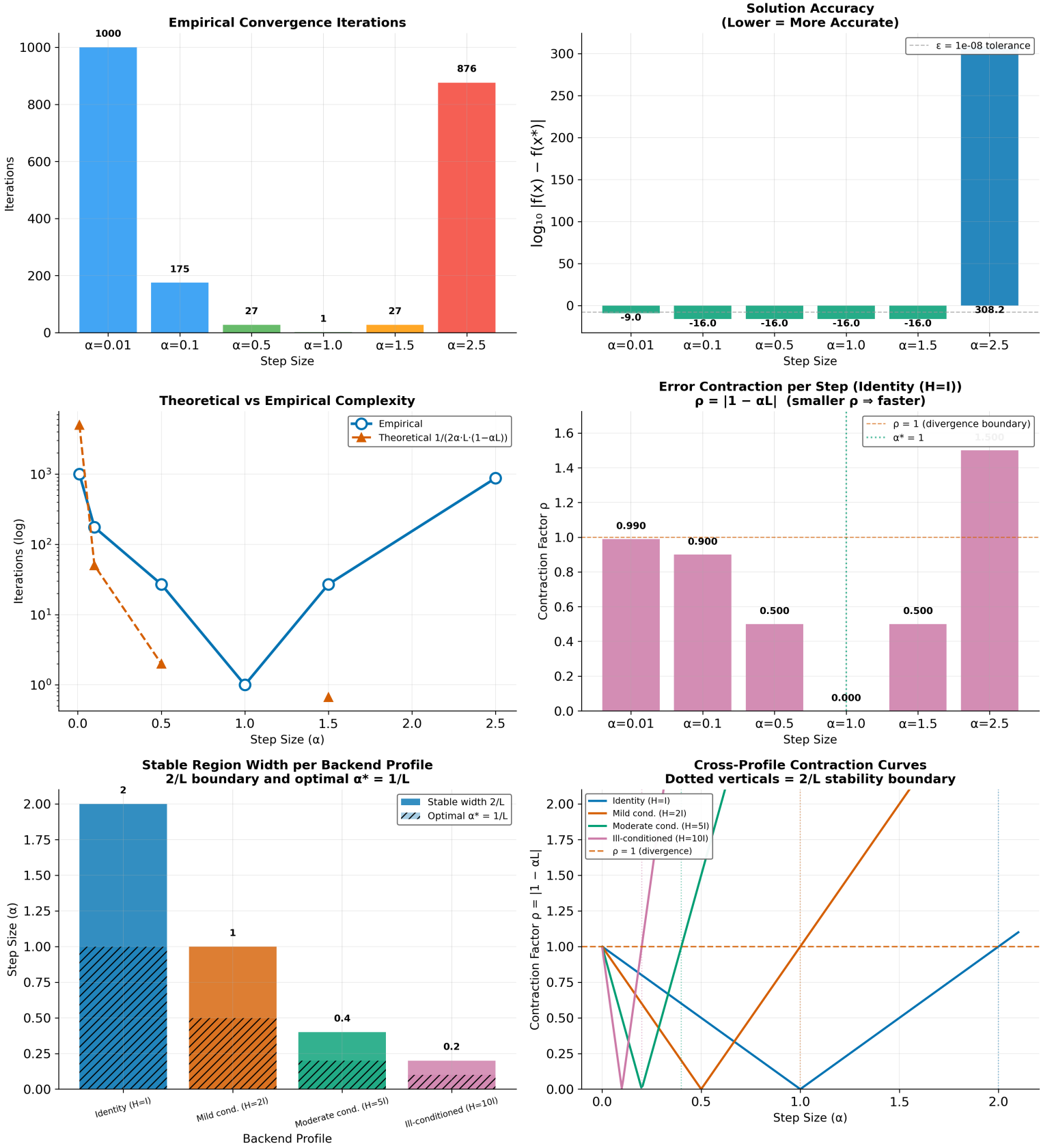
Figure 6: Six-panel diagnostic from generate_complexity_visualization() ( 3 \times 2 grid). Top left: bars give the empirical iteration count per configured \alpha , coloured by agency category; \alpha = 1.0 achieves the global minimum of 1 step(s), while \alpha = 0.01 saturates at the iteration cap N_{\max} = 1000 (slow convergence) and \alpha = 2.5 terminates early via a non-finite update (divergence). Top right: \log_{10} |f(x) - f(x^*)| at termination; the four converged rows reach \approx 10^{-16} (machine precision) while \alpha = 0.01 stops near 10^{-9} at the cap. Dashed reference at \log_{10} \varepsilon for \varepsilon = \text{experiment.convergence\_tolerance} . Middle left: empirical iterations (solid) versus the smooth proxy 1/(2\alpha L(1-\alpha L)) (dashed) on log axes — a shape comparison, not a tight count prediction for every \alpha . Middle right: per-step error contraction factor \rho = |1 - \alpha L| from the unit-Hessian linear recurrence (eq. 4); the dashed reference at \rho = 1 separates stable bars (left of it) from divergent ones (right). Bottom left: stable step-size region width 2/L per backend profile
