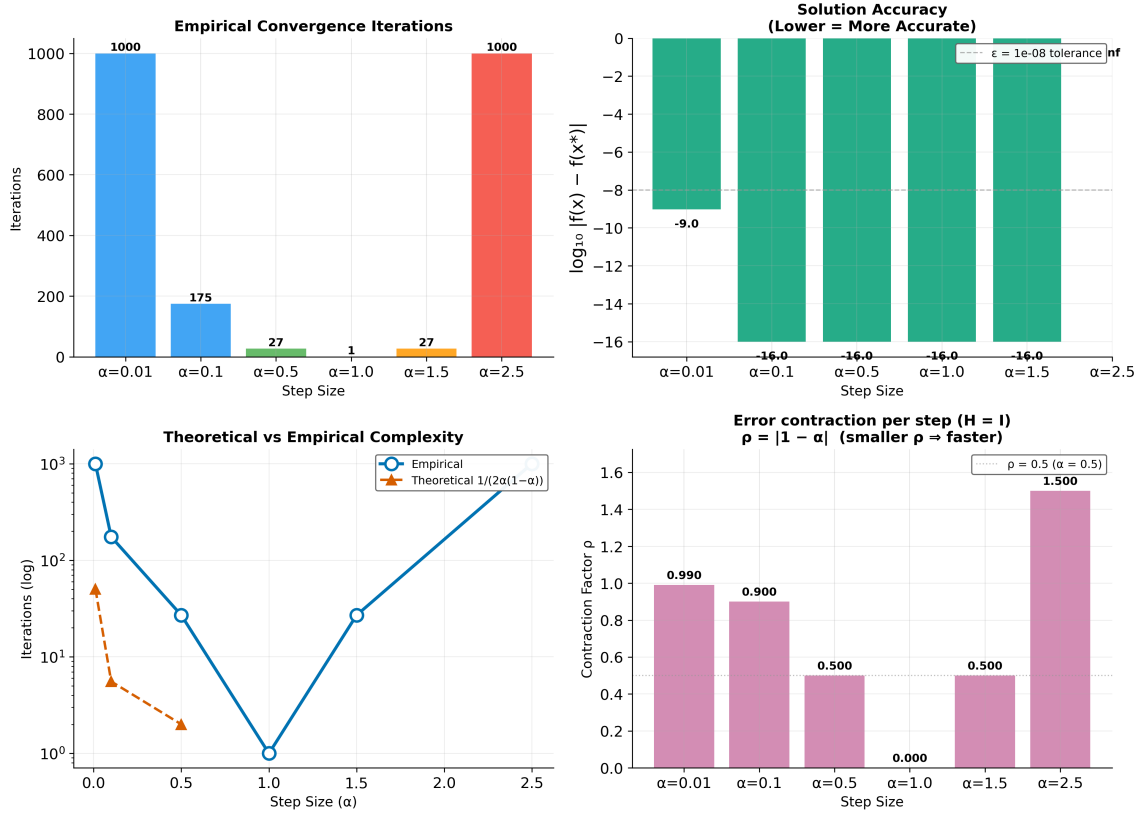
Figure 4: Four-panel diagnostic from generate_complexity_visualization() . Top left: bars give the empirical iteration count per configured \alpha , coloured by agency category; \alpha = 1.0 achieves the global minimum of 1 step(s), while \alpha = 0.01 and \alpha = 2.5 both saturate at the iteration cap N_{\max} = 1000 (slow convergence and divergence respectively). Top right: \log_{10} |f(x) - f(x^*)| at termination; the four converged rows reach \approx 10^{-16} (machine precision) while \alpha = 0.01 stops near 10^{-9} at the cap. Dashed reference at \log_{10} \varepsilon for \varepsilon = \text{experiment.convergence\_tolerance} . Bottom left: empirical iterations (solid) versus the smooth proxy 1/(2\alpha(1-\alpha)) (dashed) on log axes — a shape comparison, not a tight count prediction for every \alpha . Bottom right: per-step error contraction factor \rho = |1 - \alpha| from the unit-Hessian linear recurrence (eq. 4); the dashed reference at \rho = 1 separates stable bars (left of it) from divergent ones (right).
