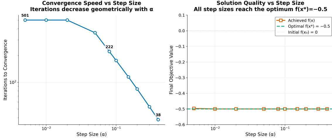
Figure 2: Sensitivity sweep produced by generate_step_size_sensitivity_plot() over an independent dense grid \alpha \in [0.005, 0.4] (15 points), distinct from the discrete experiment.step_sizes used elsewhere in this section. Left: iterations to convergence on log-log axes — the curve drops sharply from 501 iterations at the smallest \alpha (the max_iterations cap in this sub-experiment) to 38 iterations at \alpha = 0.4 , illustrating the geometric speedup as \rho(\alpha) = |1 - \alpha| shrinks. Right: final f(x) versus \alpha with horizontal reference lines at f(x_0) = 0 (initial) and f(x^*) = -0.5 (analytic optimum); every \alpha in this stable window lands on the optimum.
