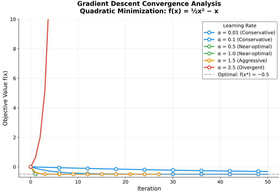
Figure 1: Objective value f(x_k) = \frac{1}{2}x_k^2 - x_k versus iteration k for gradient descent at six step sizes (legend colours follow the agency taxonomy in sec. 3: blue = conservative, green = near-optimal, orange = aggressive, red = divergent). Trajectories are produced by simulate_trajectory() in src/optimizer.py , which calls the same gradient_descent() used in tbl. 1; the upper bound on the y-axis clips the divergent \alpha = 2.5 curve so that stable trajectories remain visible. Dashed grey reference line marks the analytic optimum f(x^*) = -0.5 . Fastest configuration in this experiment: \alpha = 1.0 converges in 1 iteration(s).
