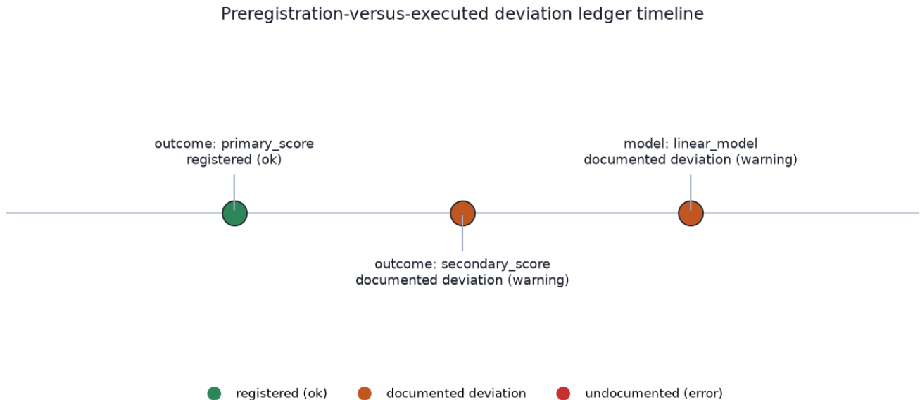
Figure 4: Preregistration-versus-executed deviation ledger timeline, rendered by plot_deviation_timeline from build_deviation_ledger and deviation_timeline . Each marker is a ledger row coloured by severity: the registered primary_score outcome is green ( ok ), while the added secondary_score endpoint and the linear_model substitution are amber ( warning , documented deviations). No marker is red because every departure carries a rationale. An undocumented departure would appear in red and invalidate the review packet.
