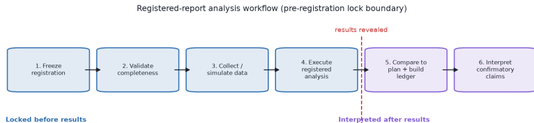
Figure 1: Registered-report analysis workflow, rendered from analysis_plan_stages() in src/registered_report/demo_study.py . The four blue stages — freeze registration, validate completeness, collect/simulate data, and execute the registered analysis — lock before results are revealed (dashed boundary). The two purple stages — compare to plan and build the deviation ledger, then interpret confirmatory claims — run only afterwards. The locks_before_results flag on each stage is what enforces the boundary in code.
