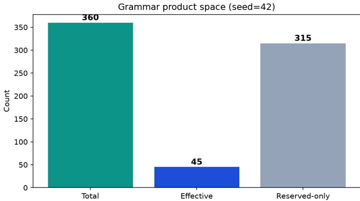
Figure 5: Total, effective, and reserved-only product size for the grammar at seed=42, generated by fig_product_space_annotation ( src/template_autopoiesis/manuscript/manuscript_figures.py ) directly from Grammar.product_size / Grammar.effective_product_size — not hand-typed.
