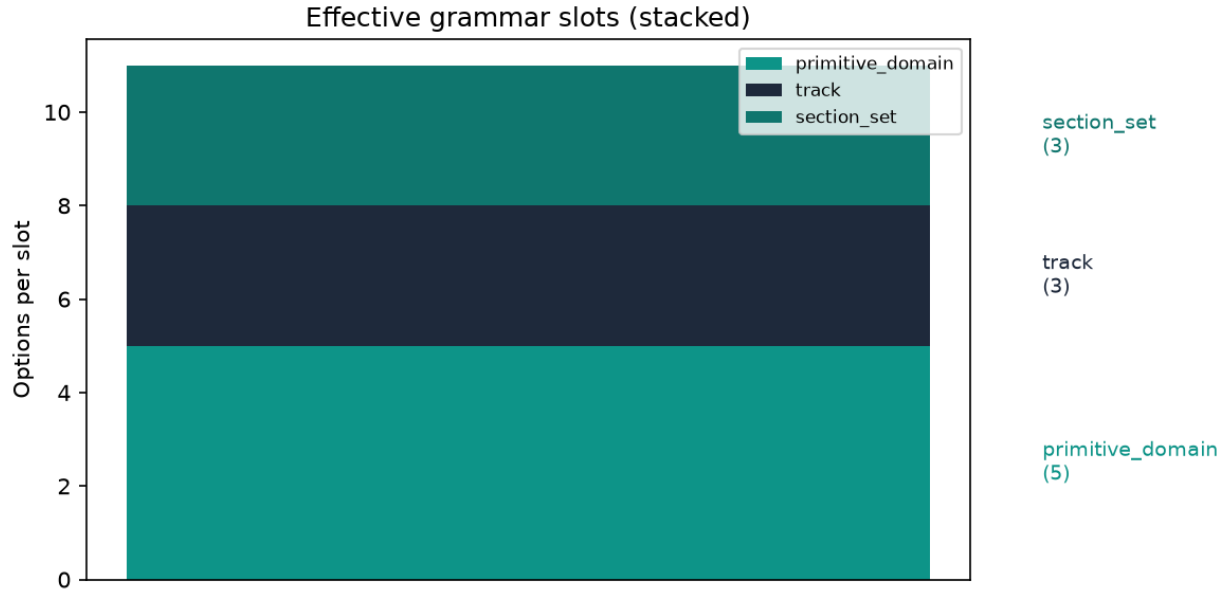
Figure 4: Options per effective grammar slot, stacked. Each band is one of the three content-determining slots; reserved presentation and sealing slots are intentionally omitted from this figure.
