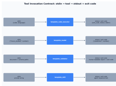
Figure 1: Invocation contract for the 4 discovered template tools: stdin payload, tool behaviour, and stdout/exit-code shape.
