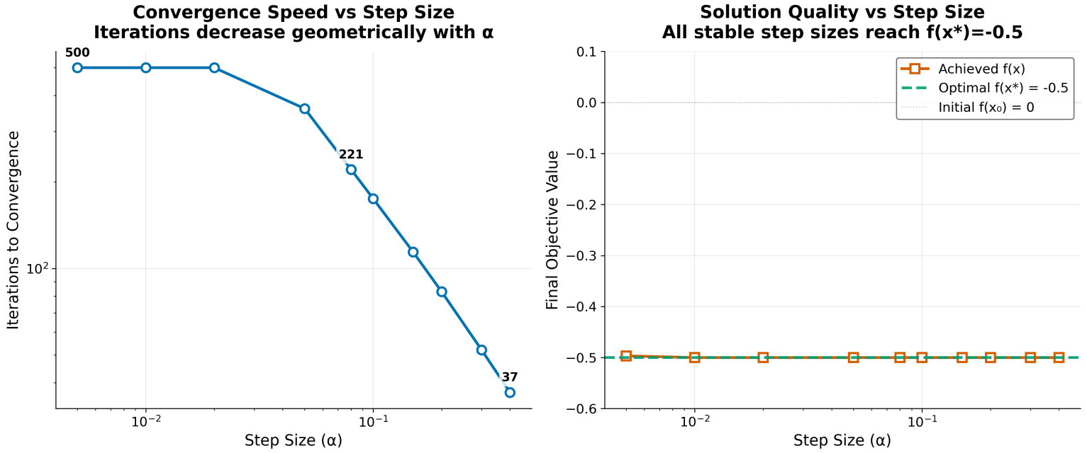
Figure 4: Sensitivity sweep produced by run_sweep over an independent dense grid \alpha \in [0.005, 0.4] (10 points), distinct from the discrete alphas used elsewhere in this section. Left: iterations to convergence on log–log axes — the curve drops sharply from 500 iterations at the smallest \alpha (the cap in this sub-experiment) to 37 iterations at \alpha = 0.4 , illustrating the geometric speedup as \rho(\alpha) = |1 - \alpha| shrinks. Right: final f(x) versus \alpha with horizontal reference lines at f(x_0) = 0 (initial) and f(x^*) = -0.5 (analytic optimum); every \alpha in this stable window lands on the optimum.
