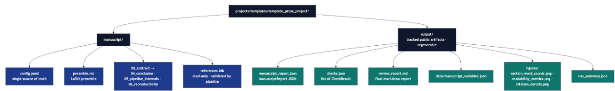
Figure 3: Mermaid diagram
