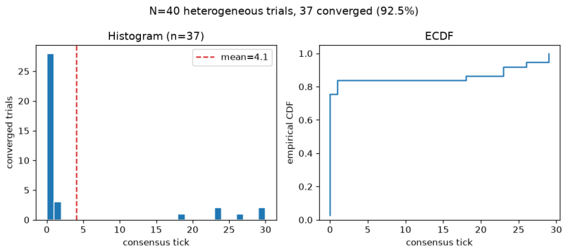
Figure 2: Convergence-tick distribution from this template's own demo statistics sweep ( src/template_formal/colony/demo.py::run_statistics_sweep , N = 40 trials, same real, heterogeneous/noisy configuration as the N = 150 test above, just smaller so the demo script stays fast): 37/40 trials converged (92.5%). Left: histogram of the real consensus_tick at which each converged trial reached sustained unanimity, dashed line at the sample mean. Right: the same distribution as an empirical CDF. This demo figure is illustrative of the shape of the real distribution at a smaller, faster N — the N = 150 Wilson-interval numbers quoted above, not this N = 40 run, are what the paper's statistical claim is bound to.
