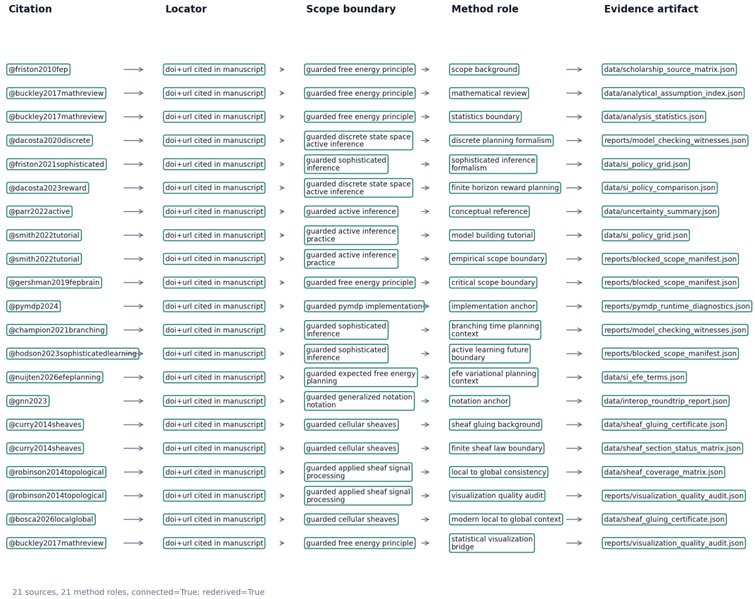
Figure 13: Scholarship source map: 21 source rows across 21 method roles and 10 source families. Connected status: true; row evidence rederived: true.
