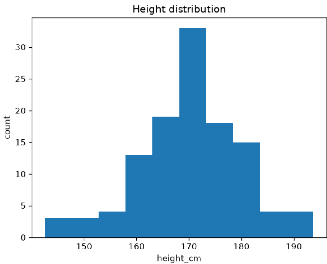
Figure 1: Height distribution: bin counts produced by histogram_data(frame, "height_cm", bins=10) in src/template_eda_notebook/eda/figures.py and plotted as a bar chart by scripts/eda_analysis.py . The bin counts sum to the number of complete-case rows; the shape is the roughly bell-shaped spread expected from the generating process.
