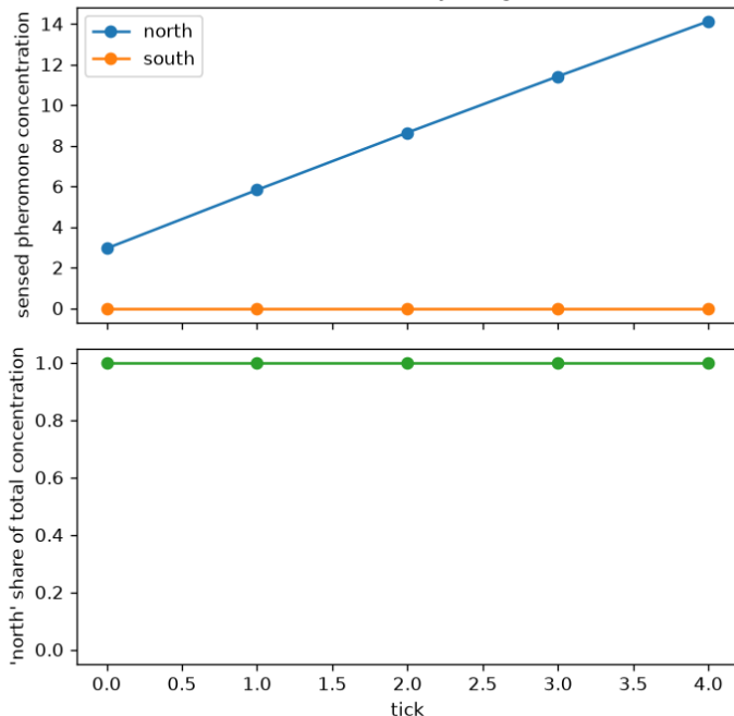
Deterministic demo colony (3 agents, 5 ticks)
