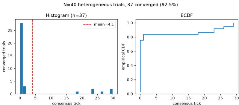
Figure 2: Convergence-tick distribution from this template's own demo statistics sweep ( src/template_formal/colony/demo.py::run_statistics_sweep , N = 40 trials, same real, heterogeneous/noisy configuration as the N = 150 test above, just smaller so the demo script stays fast): 37/40 trials converged (92.5%). Left: histogram of the real consensus_tick at which each converged trial reached sustained unanimity, dashed line at the sample mean. Right: the same distribution as an empirical CDF. This demo figure is illustrative of the shape of the real distribution at a smaller, faster N — the N = 150 Wilson-interval numbers quoted above, not this N = 40 run, are what the paper's statistical claim is bound to.
