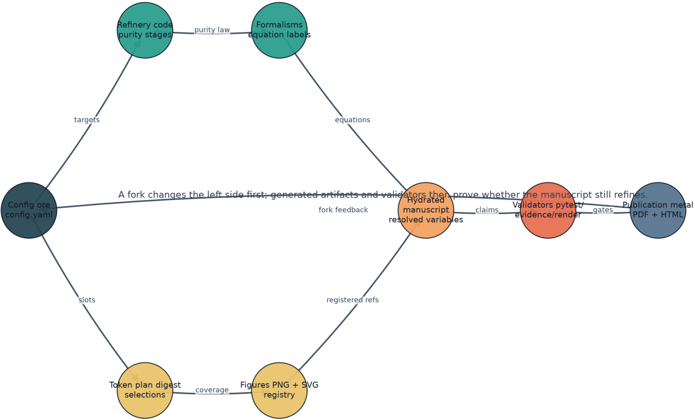
Figure 9: Implementation circuit from config-owned ore through generated manuscript artifacts and validation feedback.
