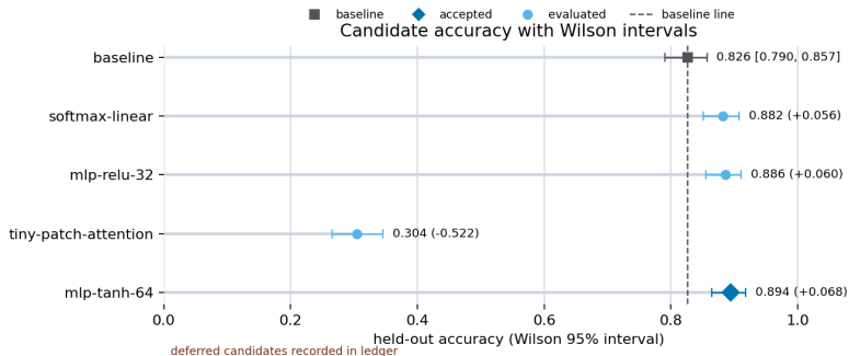
Figure 1: Held-out accuracy with Wilson intervals for the baseline and evaluated candidates from output/data/ml_candidate_intervals.json ; accepted candidate exp-mlp-tanh-64 improves accuracy from 82.6% to 89.4% on the fixed subset, with deferred proposals kept in the candidate ledger. Generation method: Lollipop accuracy comparison with Wilson interval error bars and direct labels. Registry metadata records the generation method, source artifact, and claim boundary for validation.
