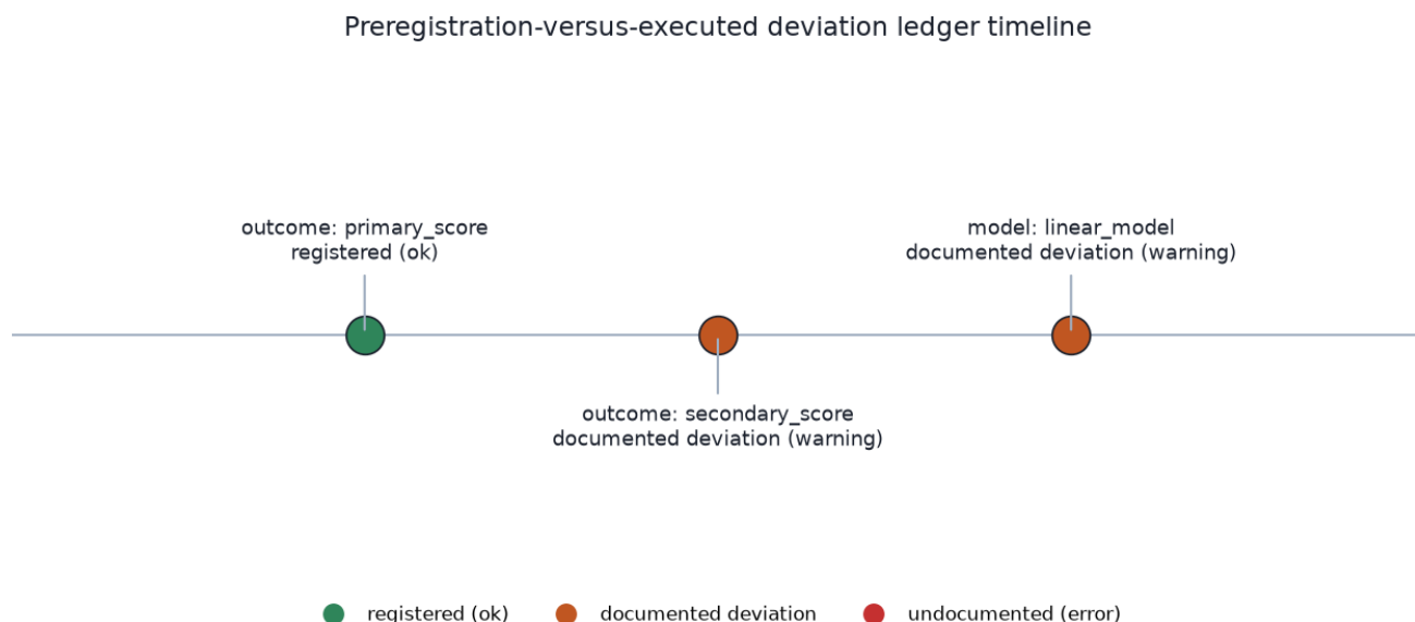
Figure 4: Preregistration-versus-executed deviation ledger timeline, rendered by plot_deviation_timeline from build_deviation_ledger and deviation_timeline . Each marker is a ledger row coloured by severity: the registered primary_score outcome is green ( ok ), while the added secondary_score endpoint and the linear_model substitution are amber ( warning , documented deviations). No marker is red because every departure carries a rationale. An undocumented departure would appear in red and invalidate the review packet.
