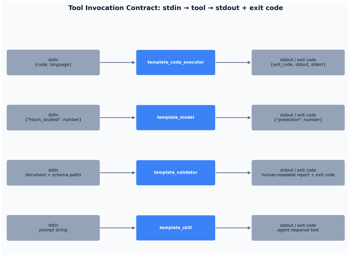
Figure 4: Invocation contract for the 4 discovered template tools: stdin payload, tool behaviour, and stdout/exit-code shape.
