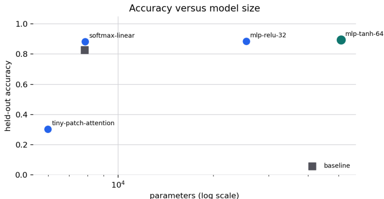
Figure 7: Parameter-count versus held-out accuracy for the baseline and evaluated candidates from output/data/ml_task_results.json; the accepted candidate is highlighted without claiming a general scaling law. Generation method: Log-parameter scatter plot against held-out accuracy. Registry metadata records the generation method, source artifact, and claim boundary for validation.
