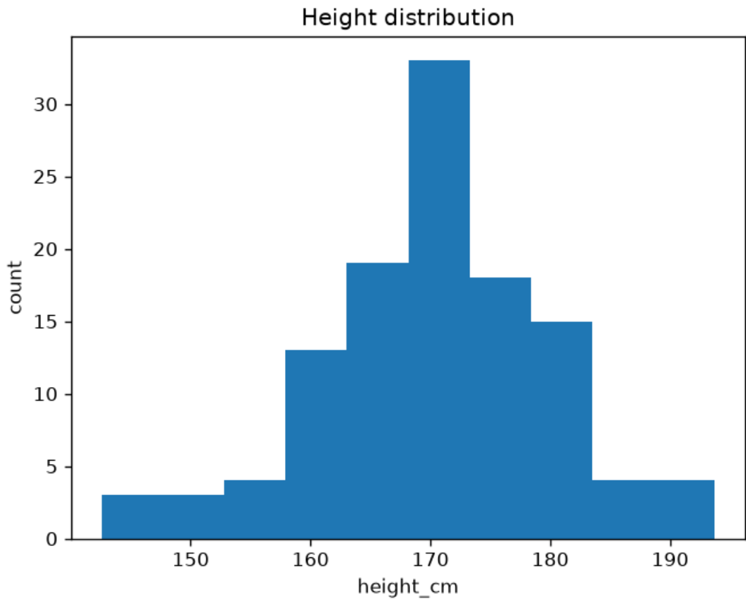
Figure 1: Height distribution: bin counts produced by in and plotted as a bar chart by . The bin counts sum to the number of complete-case rows; the shape is the roughly bell-shaped spread expected from the generating process.
