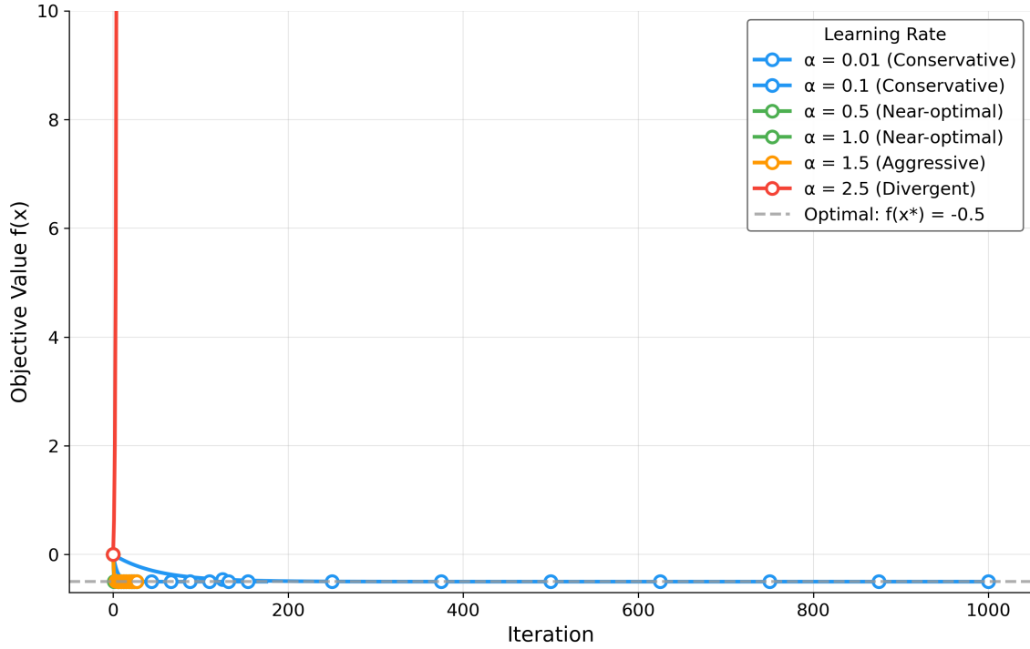
Figure 1: Objective value f(x_k) = \frac{1}{2}x_k^2 - x_k versus iteration k for gradient descent at six step sizes (legend colours follow the agency taxonomy in sec. 3: blue = conservative, green = near-optimal, orange = aggressive, red = divergent). Trajectories are produced by simulate_trajectory() in src/optimizer.py , which calls the same gradient_descent() used in tbl. 1; the upper bound on the y-axis clips the divergent \alpha = 2.5 curve so that stable trajectories remain visible. Dashed grey reference line marks the analytic optimum f(x^*) = -0.5 . Fastest configuration in this experiment: \alpha = 1.0 converges in 1 iteration(s).
