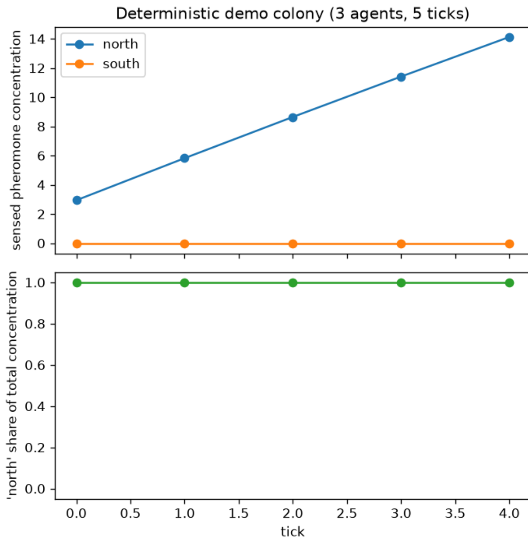
Figure 3: The deterministic demo colony’s real concentration_history ( src/template_formal/colony/demo.py::run_demo_colony , 3 agents, 2 locations, 5 ticks). Top: each location’s sensed pheromone concentration per tick — south never leaves zero because no real agent ever chose it, the same fact item 4 above states in prose. Bottom: north’s share of total concentration, constant at 1.0 from tick 0 because every agent resolves the identical free-energy tie to north on the very first tick (item 1 above) — this is the mechanism-demonstration run, presented honestly as “guaranteed by construction,” not as emergence.
