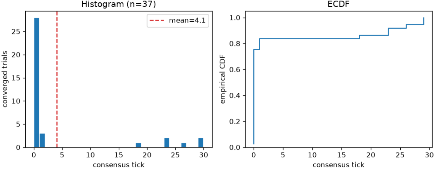
Figure 4: Convergence-tick distribution from this template’s own demo statistics sweep ( src/template_formal/colony/demo.py::run_statistics_sweep , N = 40 trials, same real, heterogeneous/noisy configuration as the N = 150 test above, just smaller so the demo script stays fast): 37/40 trials converged (92.5%). Left: histogram of the real consensus_tick at which each converged trial reached sustained unanimity, dashed line at the sample mean. Right: the same distribution as an empirical CDF. This demo figure is illustrative of the shape of the real distribution at a smaller, faster N — the N = 150 Wilson-interval numbers quoted above, not this N = 40 run, are what the paper’s statistical claim is bound to.
