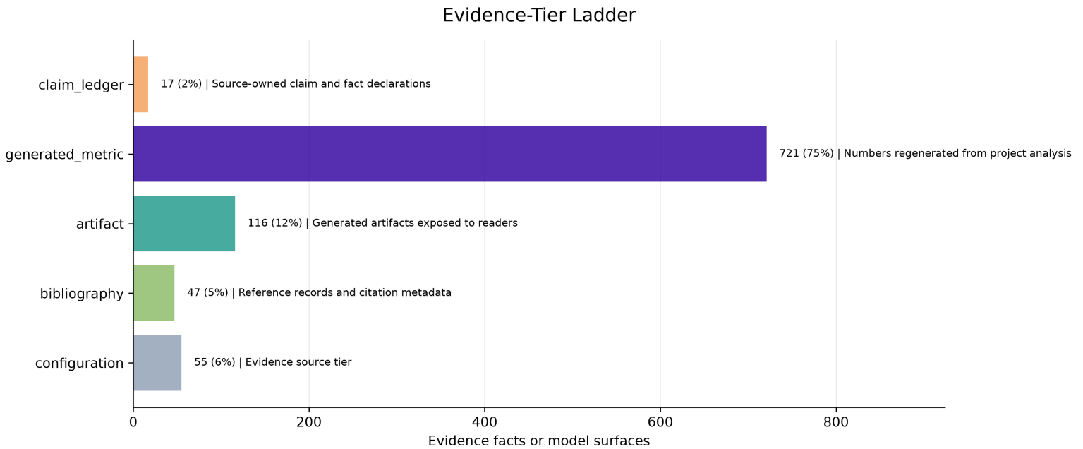
Figure 12: Evidence-tier ladder summarizing source tiers available to the shared template evidence registry.
