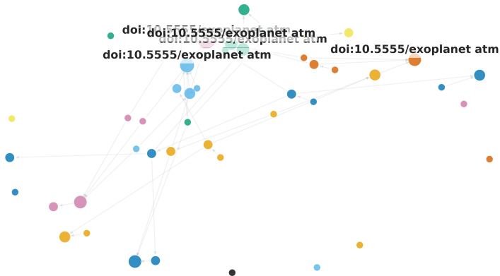
Figure 1: Citation network for Exoplanet Atmospheres. Nodes represent papers; directed edges represent citation links. Node colours indicate community membership (15 communities detected by modularity optimization). Layout uses a spring-based algorithm with a fixed seed for reproducibility.
