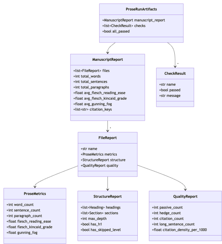
Figure 4: Mermaid diagram
