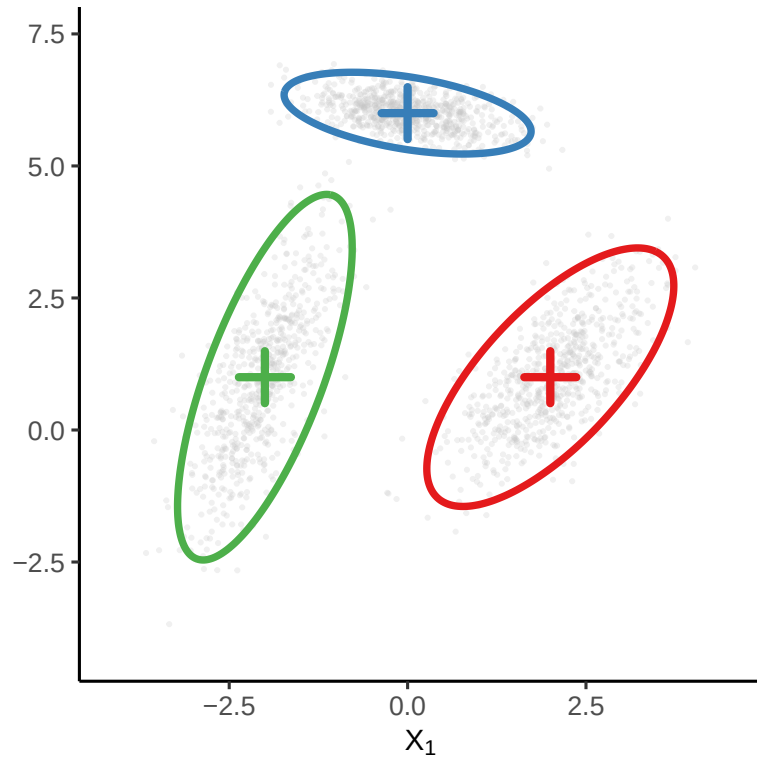
True mixture (k = 3)
