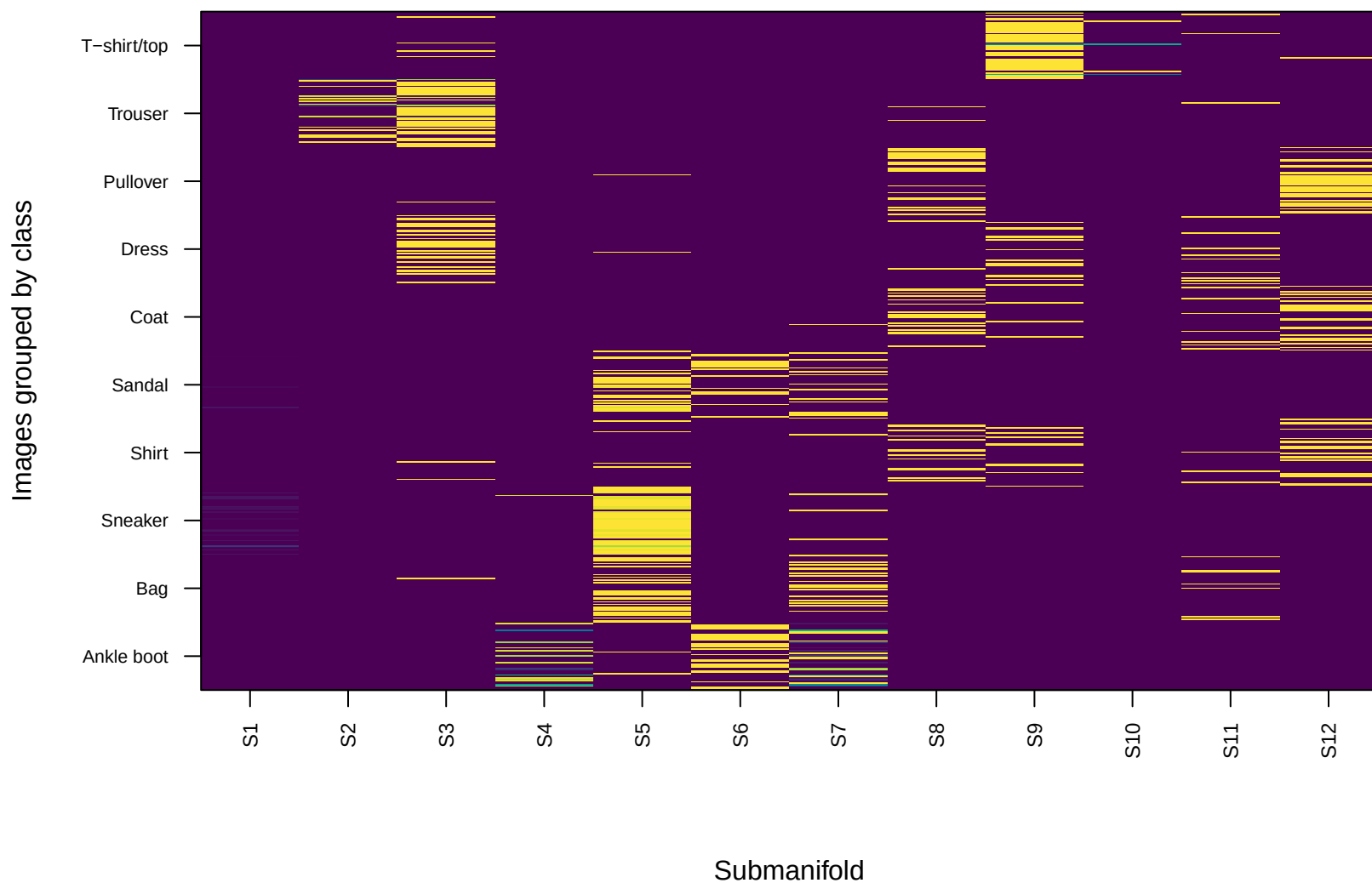
Individual responsibilities (up to 50 images per class)
