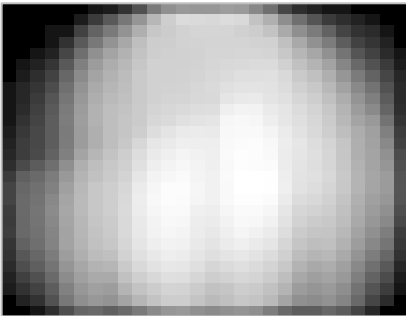
F9: Bag
