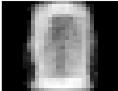
F20: Trouser
