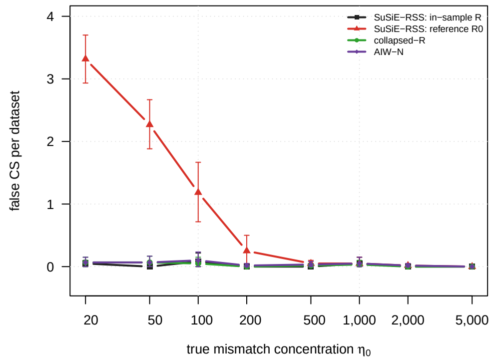
Agreement with in-sample SuSiE-RSS
