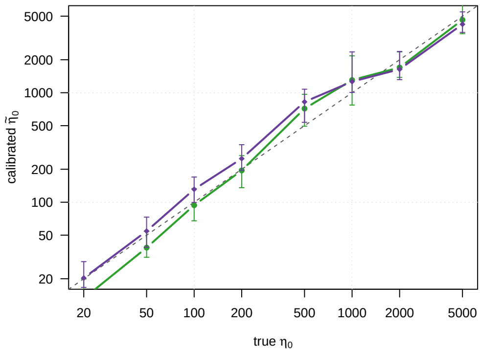
Mismatch recovery
