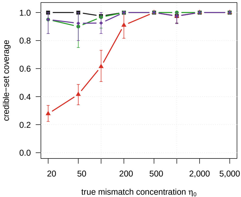
Coverage
