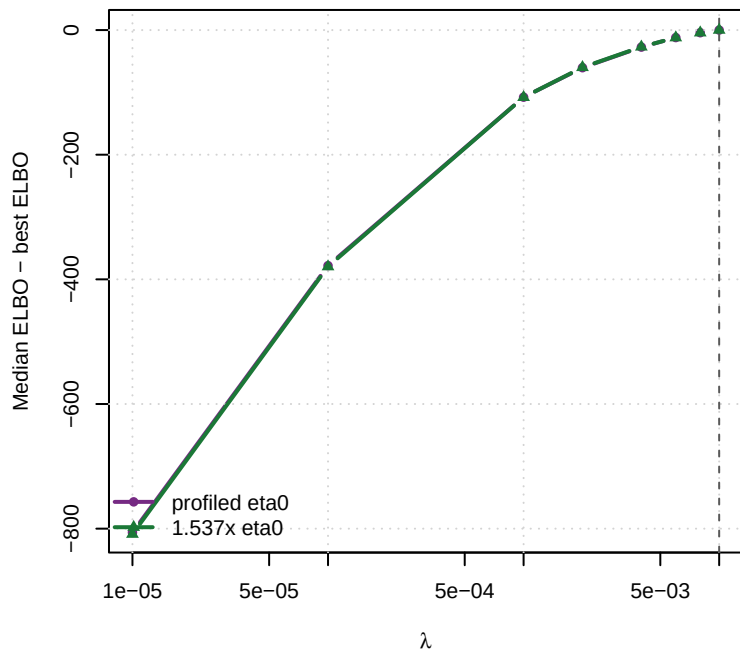
\lambda_{\text{true}} = 0.01, \eta_0 = 20
