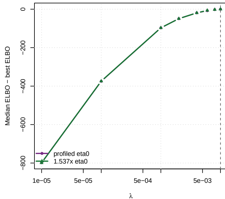
\lambda_{\text{true}} = 0.01, \eta_0 = 447
