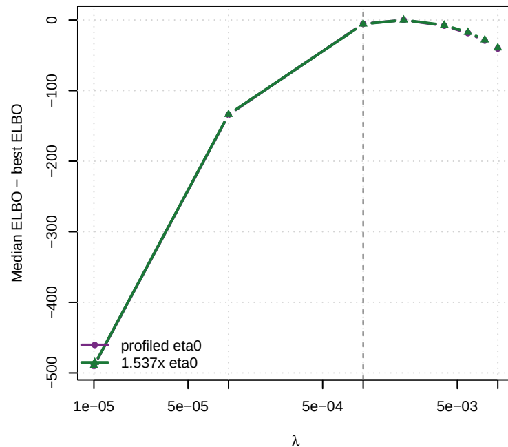
\lambda_{\text{true}} = 0.01, \eta_0 = 447
