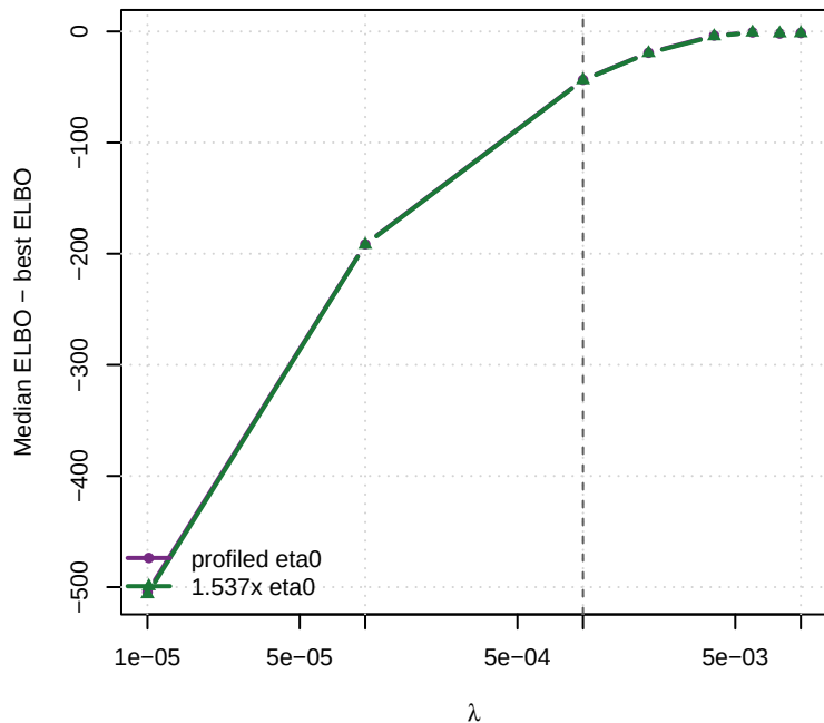
\lambda_{\text{true}} = 0.01, \eta_0 = 20
