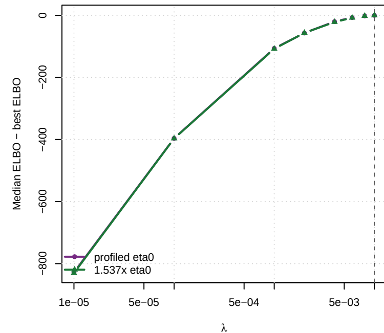
\lambda_{\text{true}} = 0.01, \eta_0 = 10000
