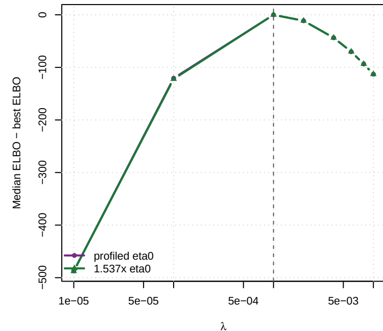
\lambda_{\text{true}} = 0.01, \eta_0 = 10000
