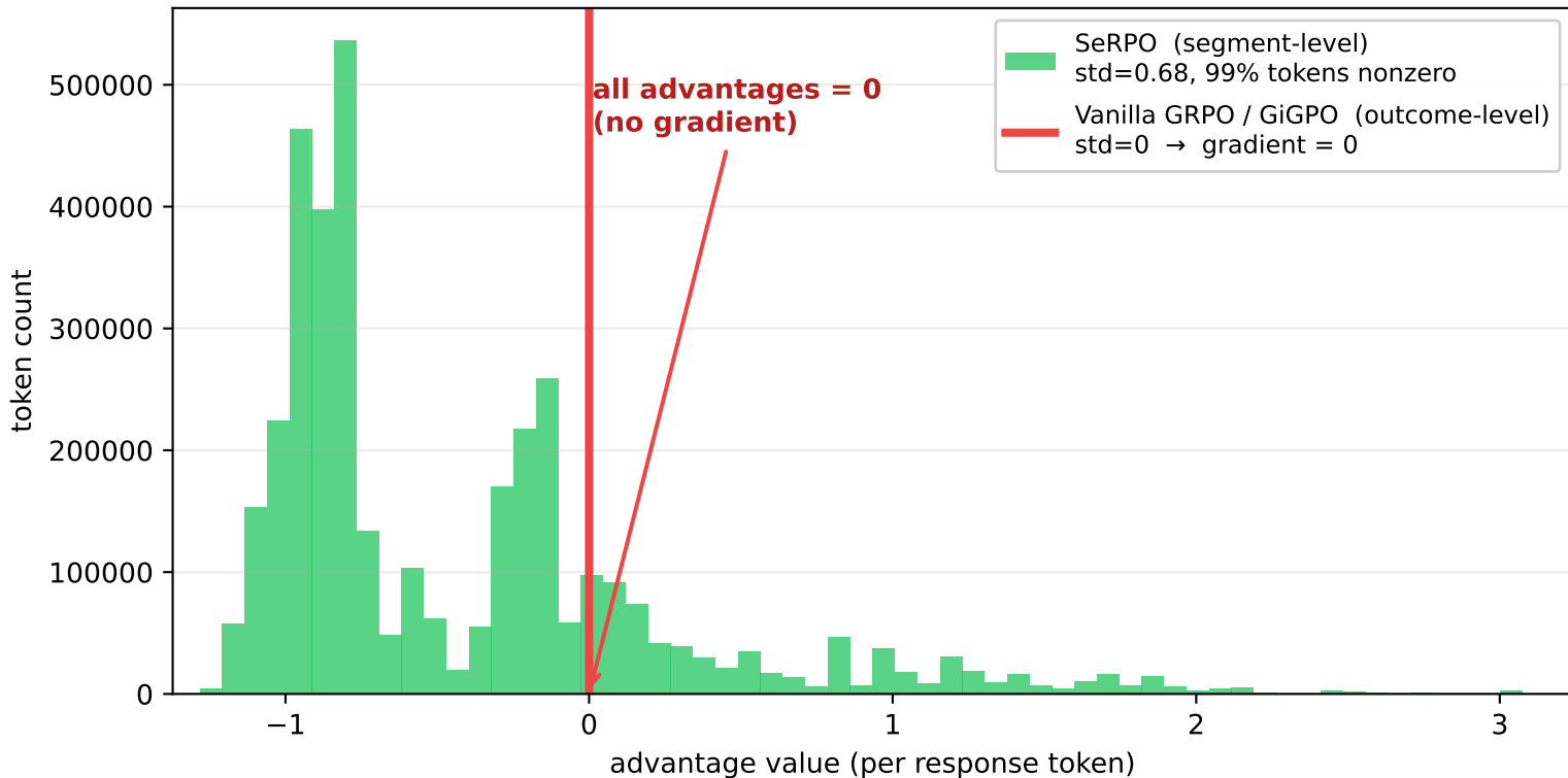
Fail-Only batch: advantage distribution 80 fail-only tasks \times 8 seeds (640 trajectories, every outcome = fail)
