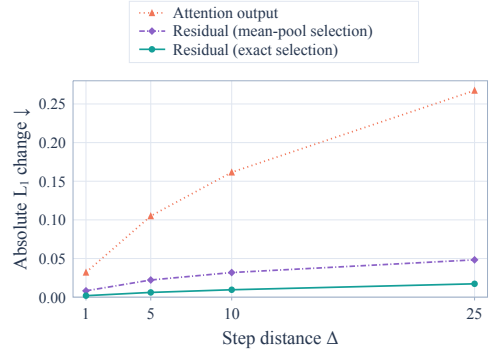
Figure 5: Absolute temporal change of attention outputs and dense-sparse residuals under token-level selection. Lower values indicate smaller absolute variation across \Delta denoising steps.
