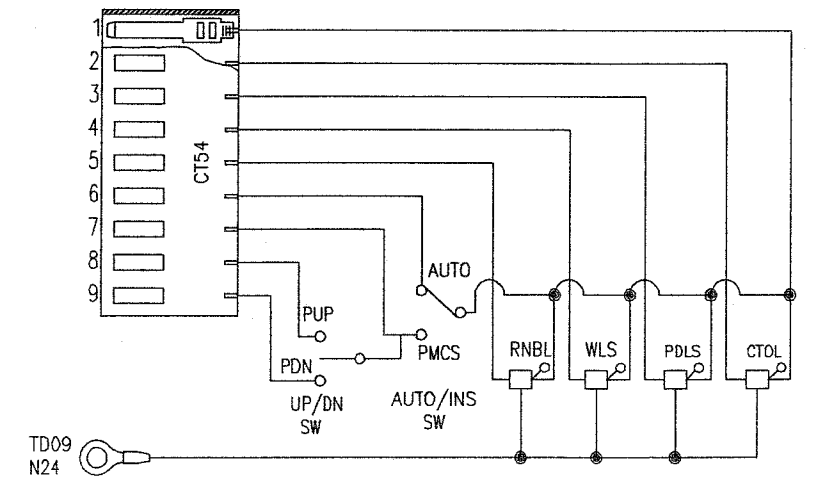
CT54 CONNECTION DIAGRAM (SIDE LOWER MRL(BASEMENT))
