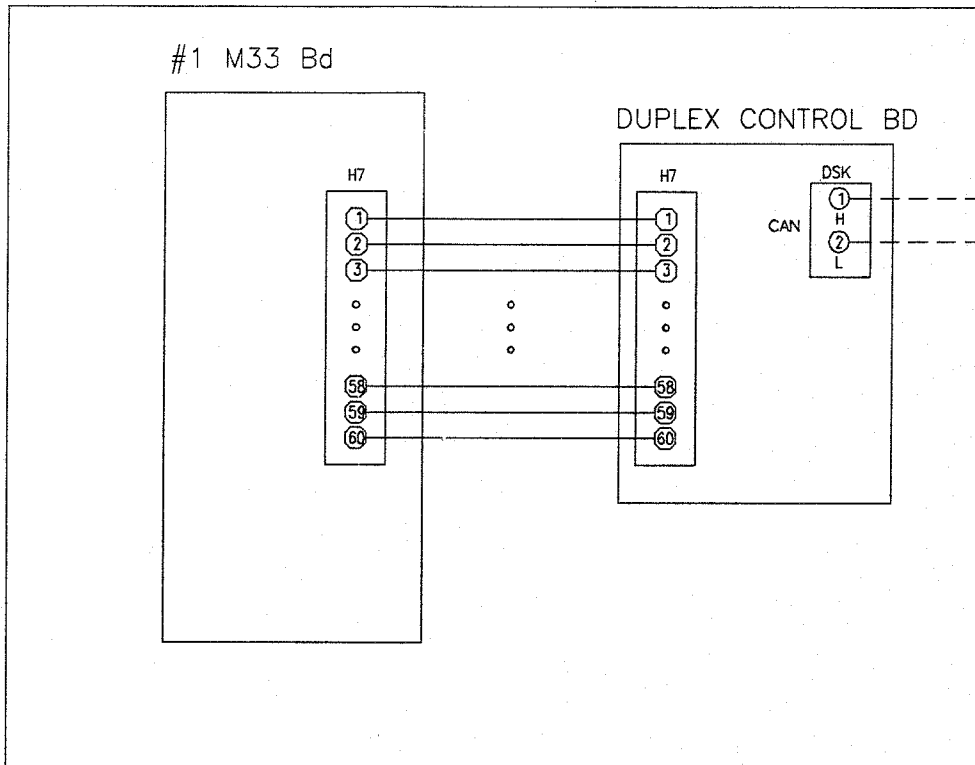
#1 CONTROL PANEL
