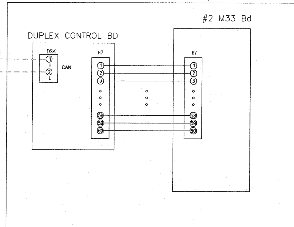
#2 CONTROL PANEL
