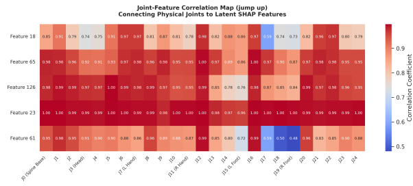
Figure 13: (a) Joint-Feature Correlation (Waving Hand) (b) Joint-Feature Correlation (Jumping) Joint-Feature Correlation maps connecting the top 5 SHAP features (latent space) directly to the physical joint representations (spatial dimensions).
