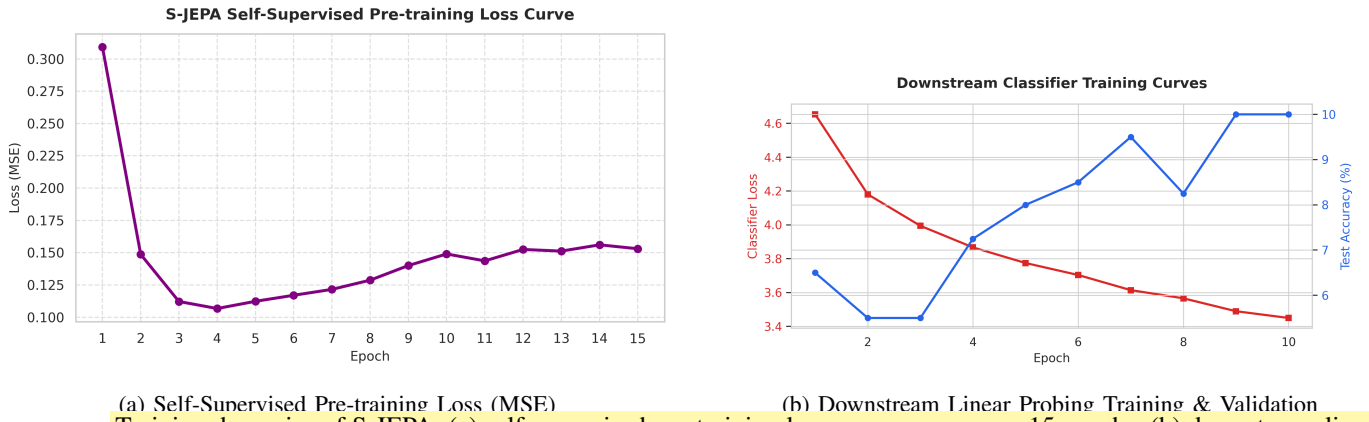
Figure 15: Training dynamics of S-JEPA: (a) self-supervised pre-training loss convergence over 15 epochs, (b) downstream linear probing learning curves over 10 epochs.
