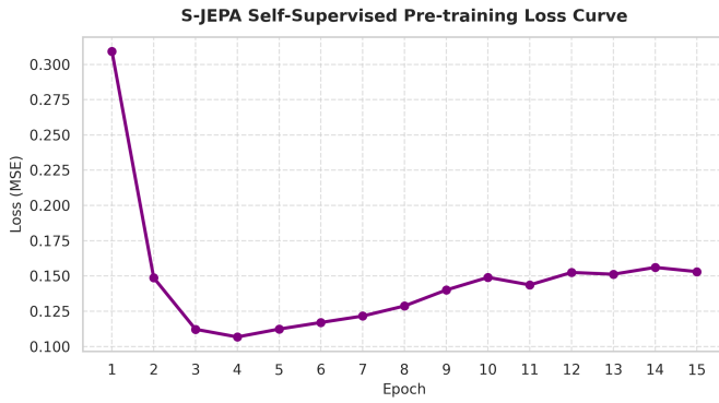
Figure 15: Training dynamics of S-JEPA: (a) self-supervised pre-training loss convergence over 15 epochs, (b) downstream linear probing learning curves over 10 epochs.
