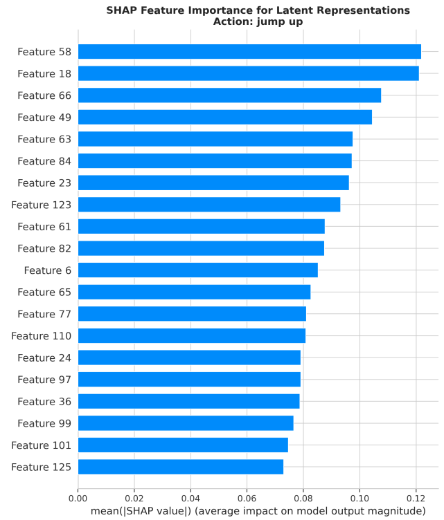
(a) Feature contribution for Waving hand (b) Feature contribution for Jumping Figure 11: SHAP Feature Importance chart explaining the contribution of S-JEPA latent features to classification decisions.
