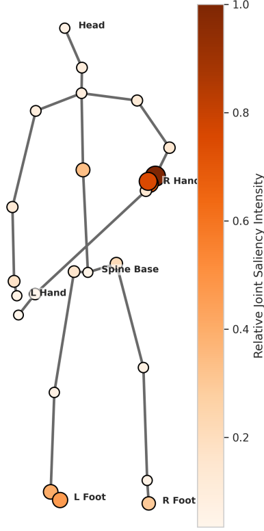
(a) Saliency of Waving hand action
