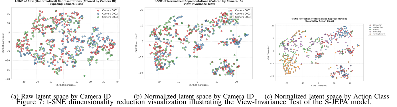
Figure 7: t-SNE dimensionality reduction visualization illustrating the View-Invariance Test of the S-JEPA model.
