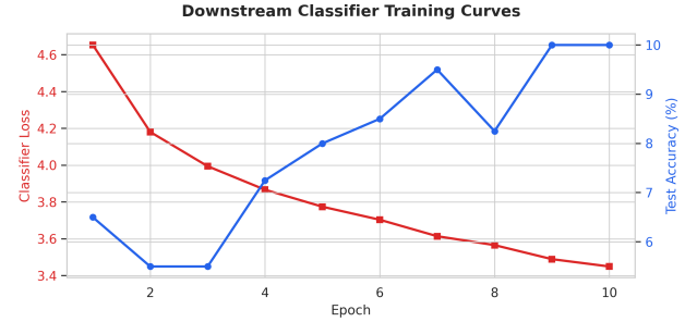
Figure 15: Training dynamics of S-JEPA: (a) self-supervised pre-training loss convergence over 15 epochs, (b) downstream linear probing learning curves over 10 epochs.
