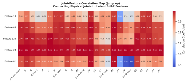
(a) Joint-Feature Correlation (Waving Hand) (b) Joint-Feature Correlation (Jumping) Figure 12: Joint-Feature Correlation maps connecting the top 5 SHAP features (latent space) directly to the physical joint representations (spatial dimensions).
