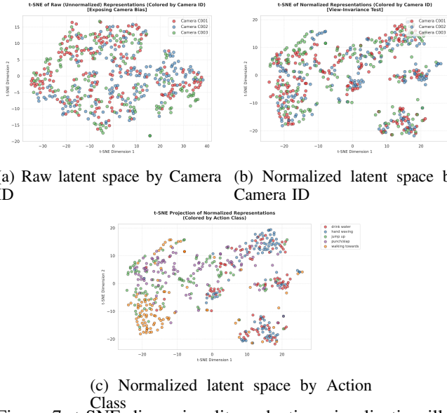
Figure 7: t-SNE dimensionality reduction visualization illustrating the View-Invariance Test of the S-JEPA model.
