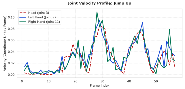
(a) Waving Action (b) Jumping Action Figure 3: Line chart visualization comparing the real-time velocity kinetic variations of different joints.
