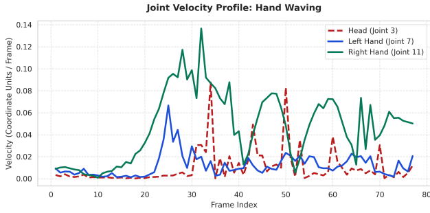
(a) Waving Action (b) Jumping Action Figure 3: Line chart visualization comparing the real-time velocity kinetic variations of different joints.
