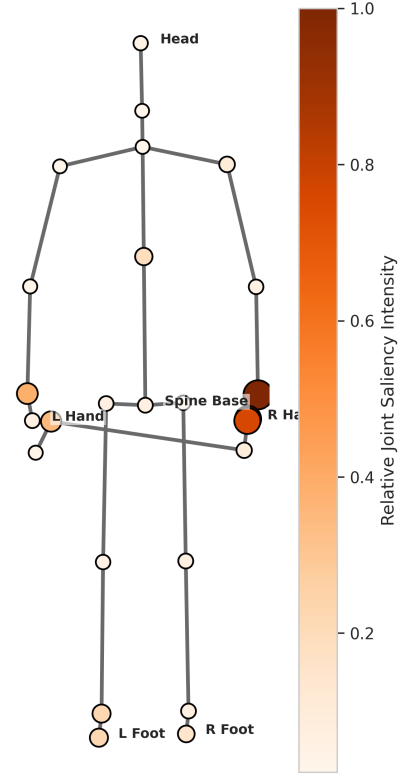
Gradient Saliency Joint Overlay Action: Jumping
