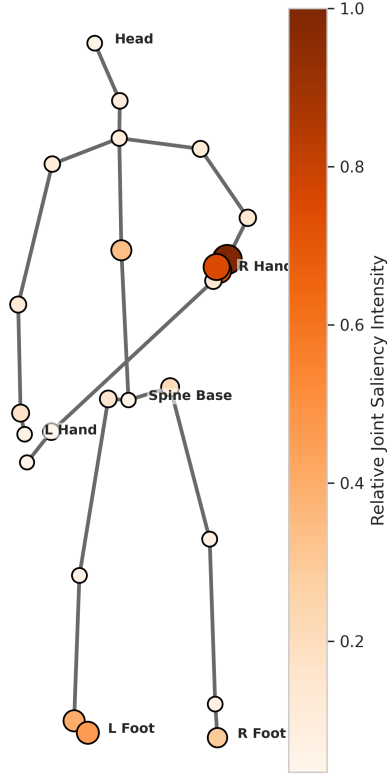
Gradient Saliency Joint Overlay Action: Waving hand
