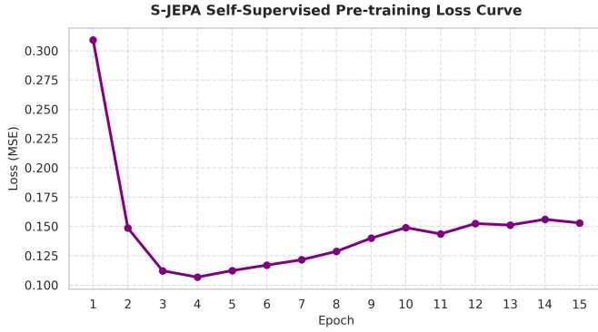
(a) Self-Supervised Pre-training Loss (MSE)
