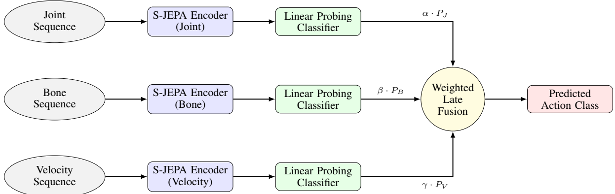
Figure 11: The Multi-stream Late Fusion pipeline diagram of the S-JEPA model.
