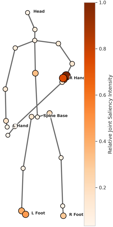
(a) Saliency of Waving hand action
