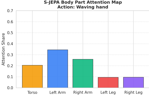
Figure 9: Attention Share maps distributed across human body parts by the S-JEPA model for each action. (a) Waving hand action (b) Jumping action
