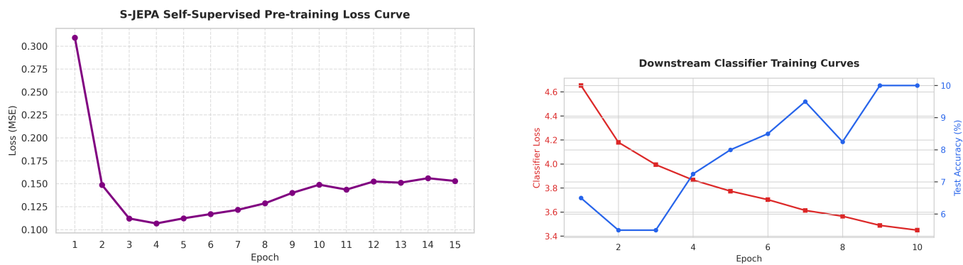
Figure 15: Training dynamics of S-JEPA: (a) self-supervised pre-training loss convergence over 15 epochs, (b) downstream linear probing learning curves over 10 epochs.
