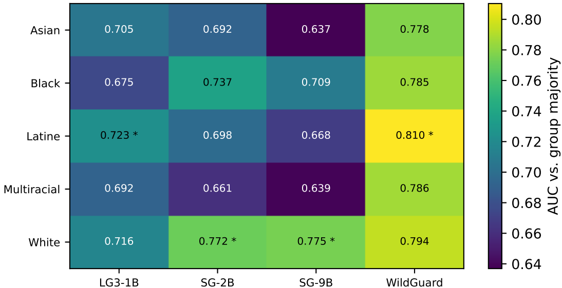
Per-group ranking alignment (* = best-tracked group)
